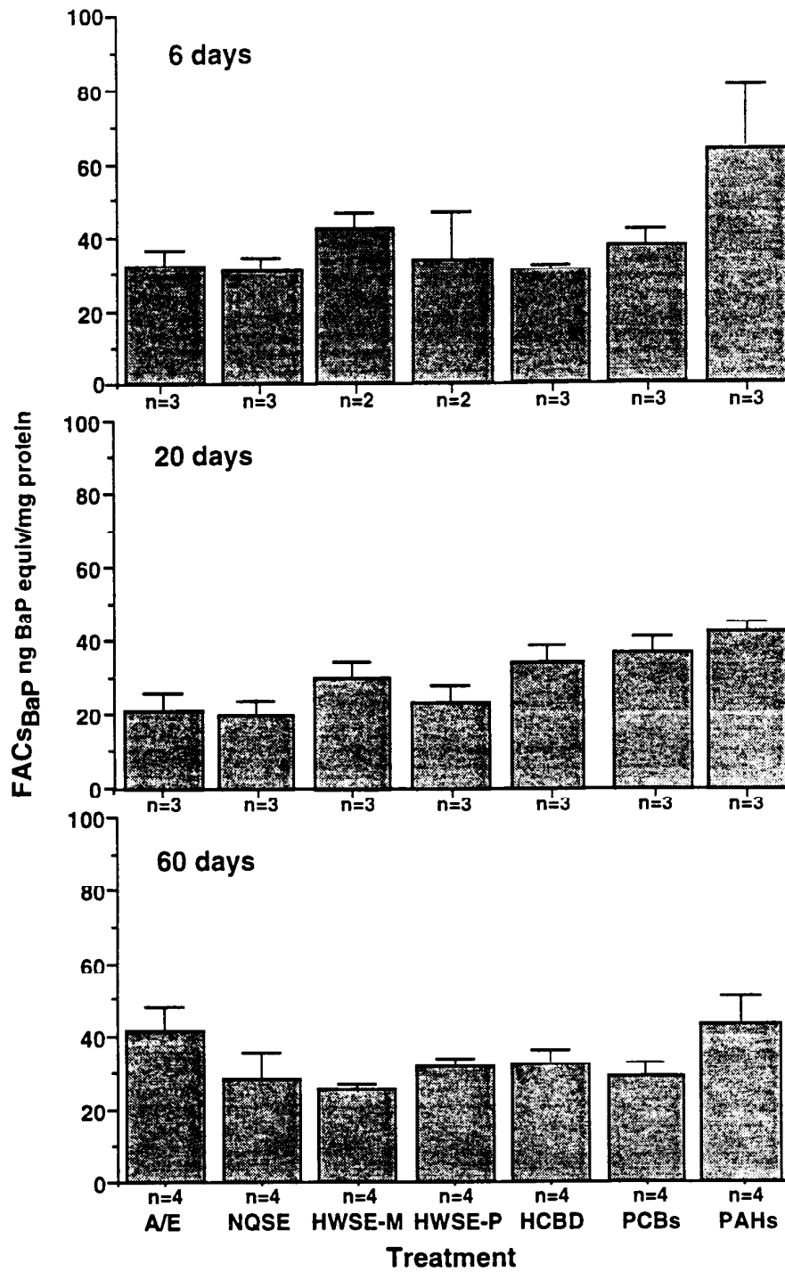
Figure 5. Biliary FACs in juvenile chinook salmon exposed to selected chemical contaminants. Values are mean \pm SE. n = number of analyses. ppb = parts per billion. A/E = acetone/ emulphor injection vehicle, NQSE = Nisqually sediment extract, HWSE-M = Hylebos Waterway sediment extract- sediment extracted with methylene chloride, HWSE-P = Hylebos Waterway sediment extract with pentane, PCBs = polychlorinated biphenyls.
