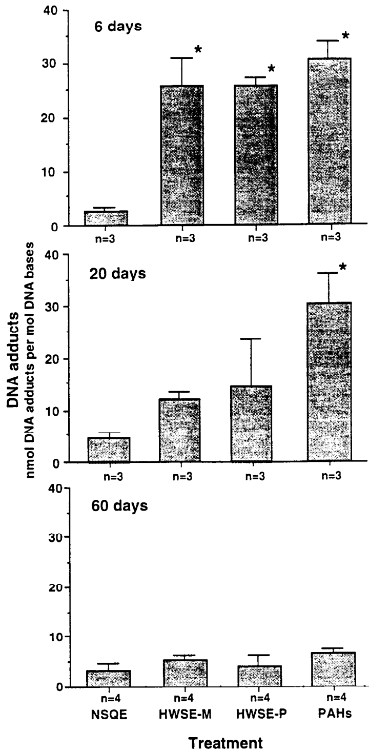
Figure 7. Hepatic DNA adducts in juvenile chinook salmon exposed to selected chemical contaminants. Values are mean \pm SE. n = number of analyses.
