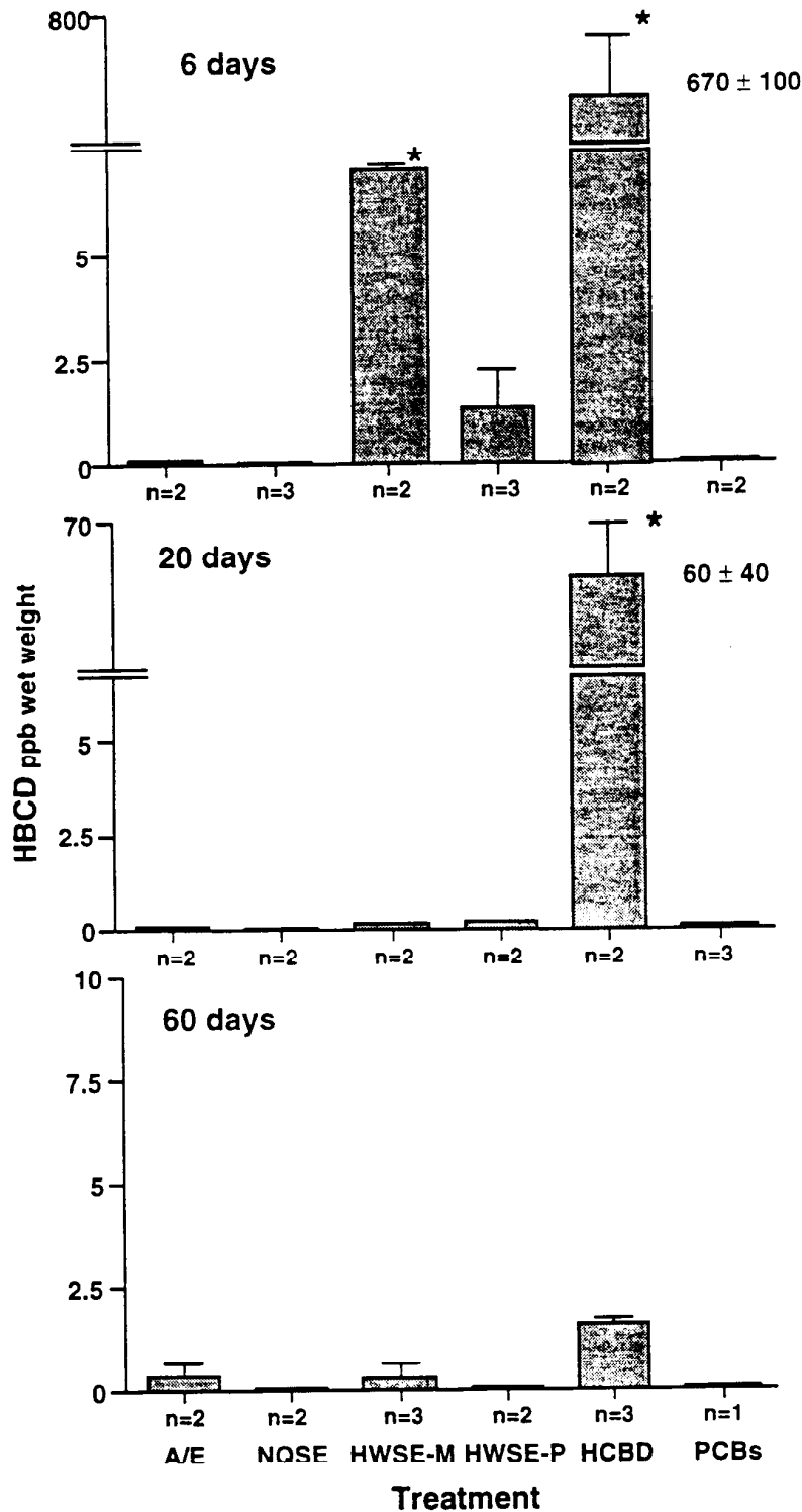
Figure 4. Whole body HBCD concentrations in juvenile chinook salmon exposed to selected chemical contaminants. Values are mean \pm SE. n = number of analyses. * = Value is significantly different from A/E and NQSE groups. ppb = parts per billion. A/E = acetone/ emulphor injection vehicle, NQSE = Nisqually sediment extract, HWSE-M = Hylebos Waterway sediment extracted with methylene chloride, HWSE-P = Hylebos Waterway sediment extracted with pentane, HCB = hexachlorobutadiene, PCBs = polychlorinated biphenyls.
