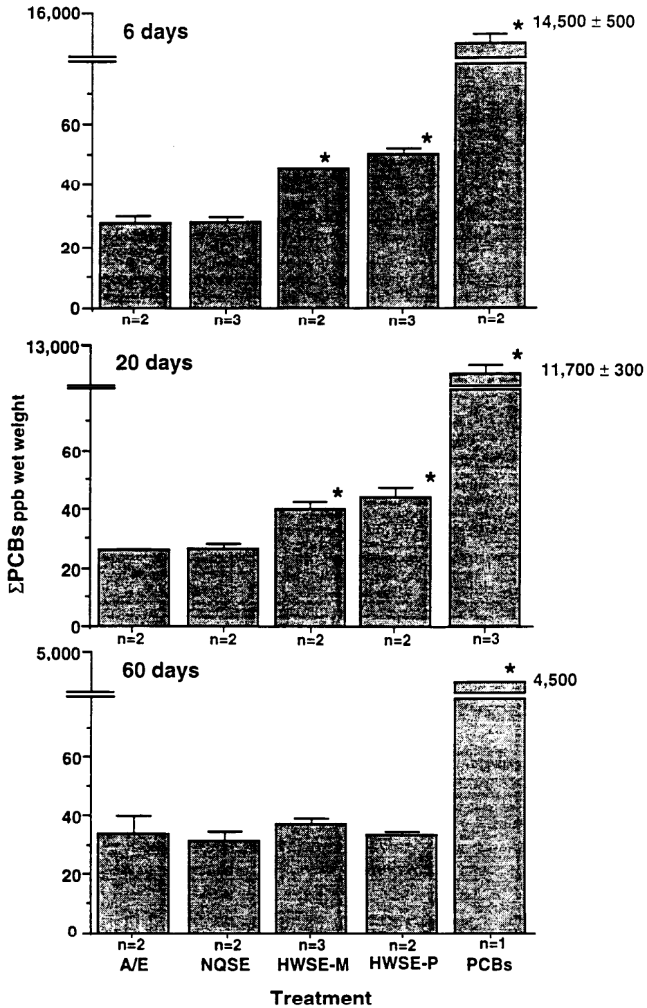
Figure 2. Whole body \Sigma PCBs in juvenile chinook salmon exposed to selected chemical contaminants. Values are mean \pm SE. n = number of analyses. * = Value is significantly different from A/E and NQSE groups. ppb = parts per billion. A/E = acetone/ emulphor injection vehicle, NQSE = Nisqually sediment extract, HWSE-M = Hylebos Waterway sediment extracted with methylene chloride, HWSE-P = Hylebos Waterway sediment extracted with pentane, PCBs = polychlorinated biphenyls.
