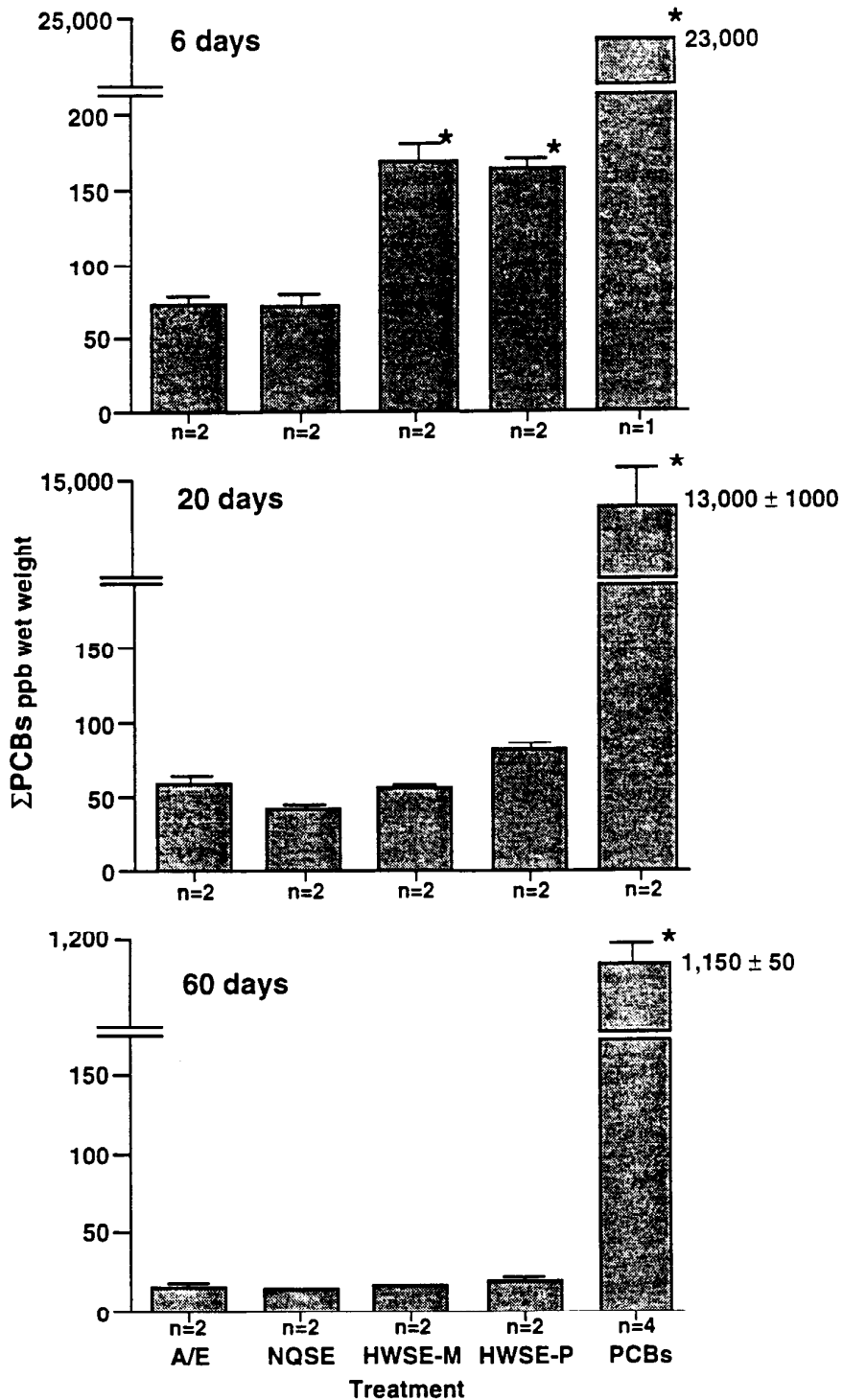
Figure 1. Hepatic \Sigma PCBs in juvenile chinook salmon exposed to selected chemical contaminants. Values are mean \pm SE. n = number of analyses. * = Number is significantly different from A/E and NQSE groups. ppb = parts per billion. A/E = acetone/ emulphor injection vehicle, NQSE = Nisqually sediment extract, HWSE-M = Hylebos Waterway sediment extract- sediment extracted with methylene chloride, HWSE-P = Hylebos Waterway sediment extracted with pentane, PCBs = polychlorinated biphenyls.
