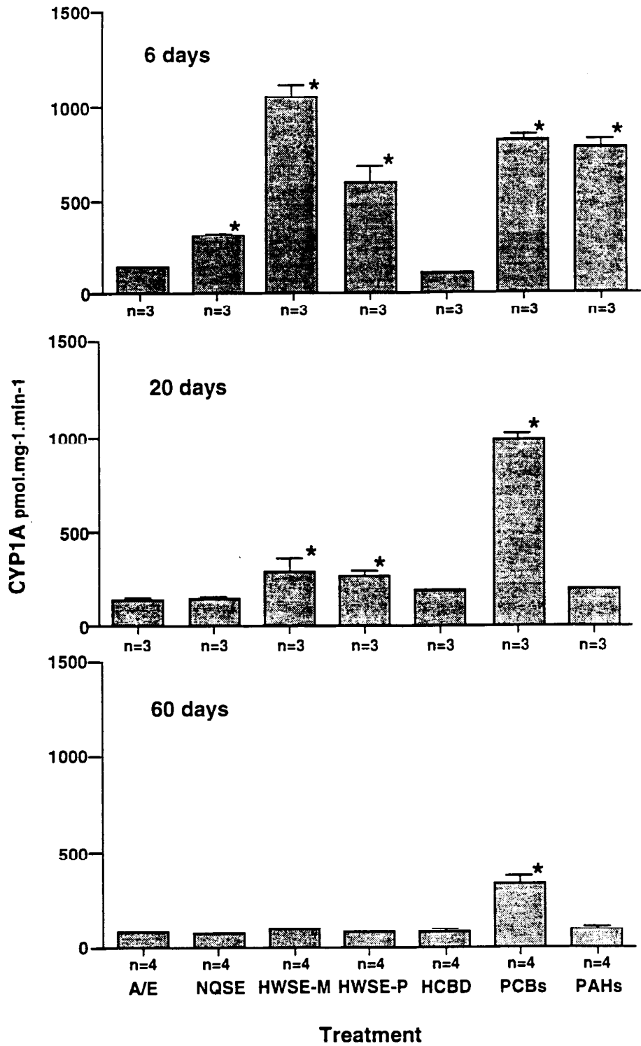
Figure 6. Hepatic cytochrome P4501A (CYP1A) activity in juvenile chinook salmon exposed to selected chemical contaminants. Values are mean \pm SE. n = number of analyses. * = Value is significantly different from A/E and NQSE groups. ppb = parts per billion. A/E = acetone/ emulphor injection vehicle, NQSE = Nisqually sediment extract, HWSE-M = Hylebos Waterway sediment extracted with methylene chloride, HWSE-P = Hylebos Waterway sediment extracted with pentane, HCBd = hexachlorobutadiene. PCBs = polychlorinated biphenyls. PAHs = polynuclear aromatic hydrocarbon.
