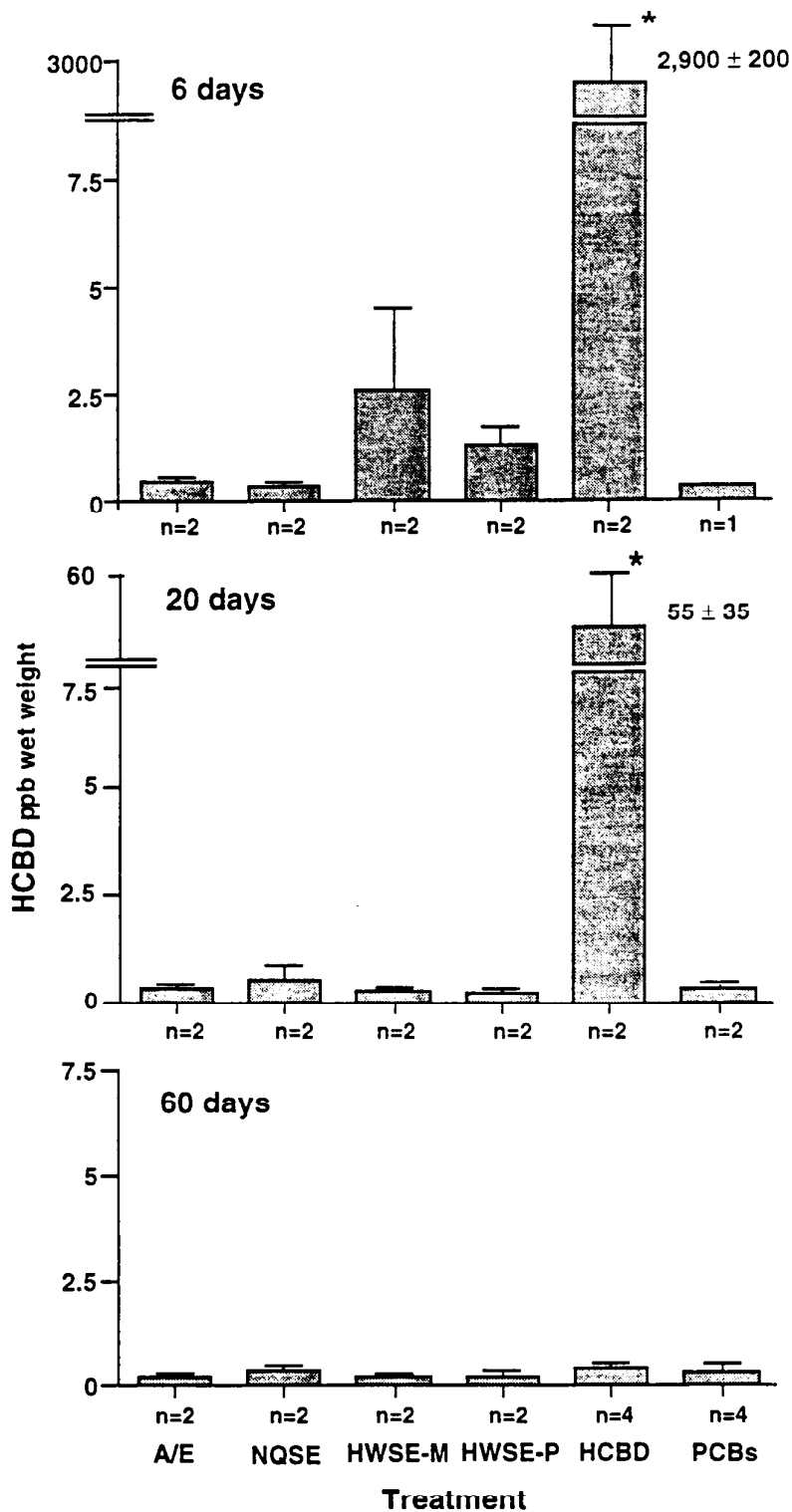
Figure 3. Hepatic HCBd concentrations in juvenile chinook salmon exposed to selected chemical contaminants. Values are mean \pm SE. n = number of analyses. * = Value is significantly different from A/E and NQSE groups. ppb = parts per billion. A/E = acetone/ emulphor injection vehicle, NQSE = Nisqually sediment extract, HWSE-M = Hylebos Waterway sediment extracted with methylene chloride, HWSE-P = Hylebos Waterway sediment extracted with pentane, HCBd = hexachlorobutadiene. PCBs = polychlorinated biphenyls.
