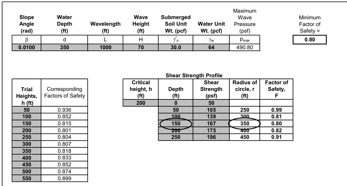
Figure C13. Identification of properties of the critical slip circle
