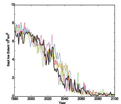
Fig. 2. Projections of Arctic sea ice extent from multiple National Center for Atmospheric Research model ensemble members. Redrawn from Holland et al. [2006].
