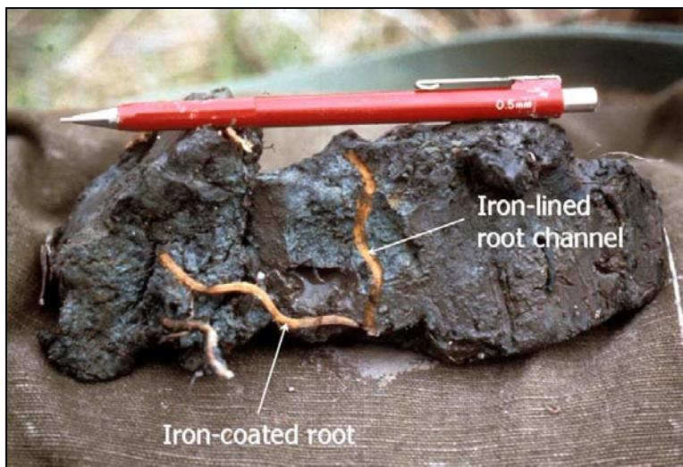
Figure 40. Iron-oxide plaque (orange coating) on a living root. Iron also coats the channel or pore from which the root was removed.
