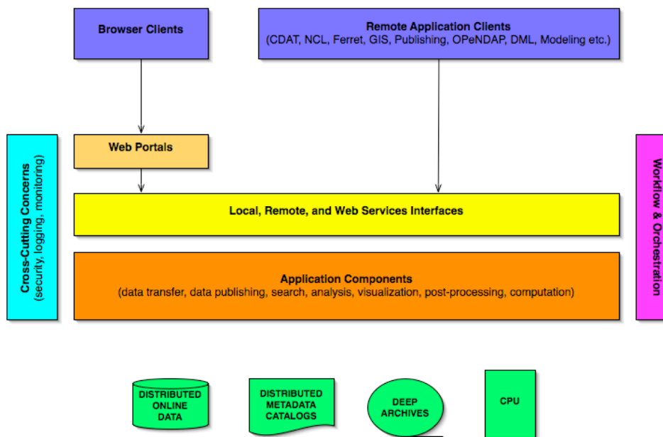
Figure 2: Future ESG-CET Architecture
