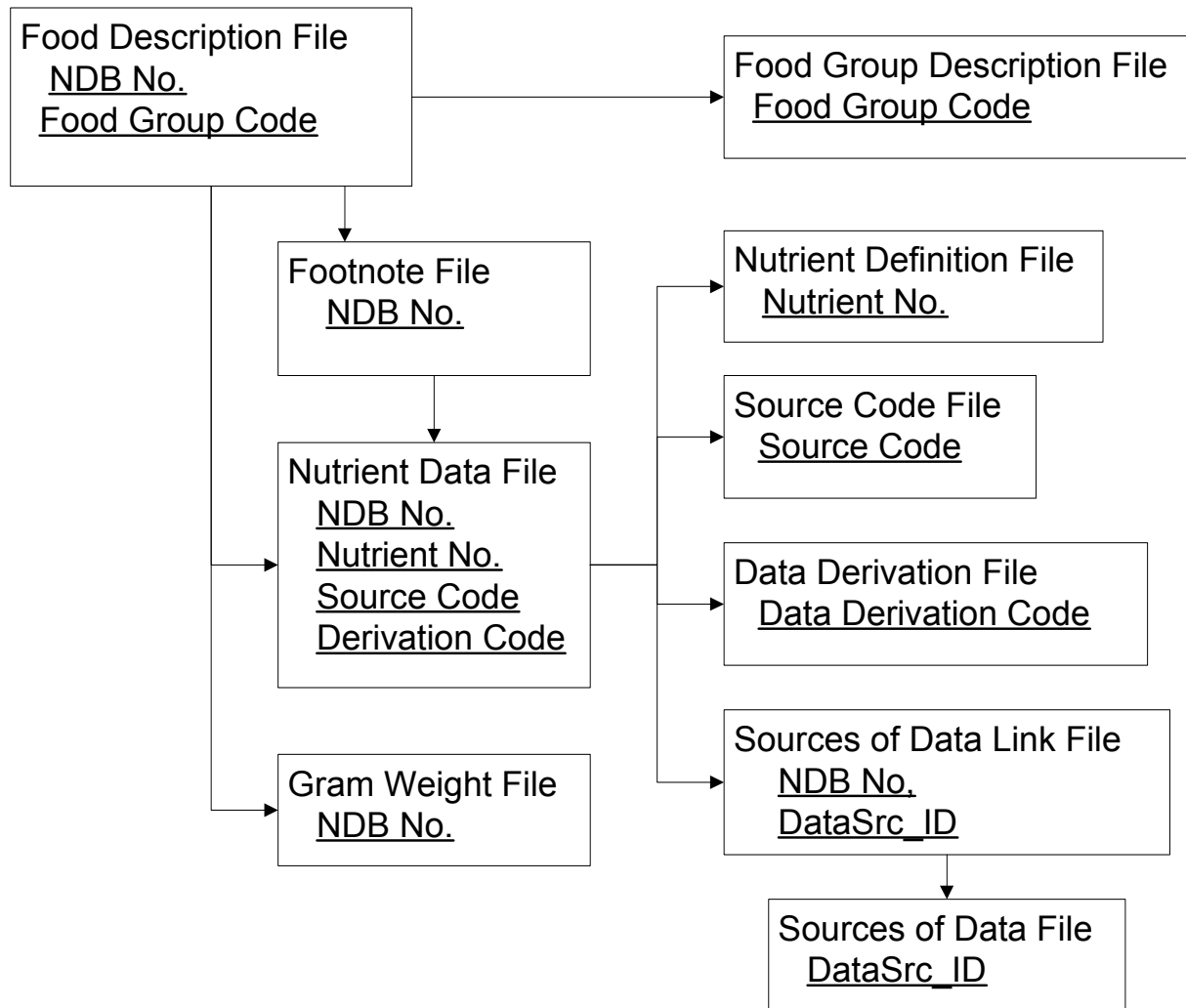
Figure 1. Relationship among files in the USDA National Nutrient Database for Standard Reference
