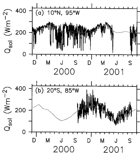
Fig. 3. Daily averaged incoming solar radiation (black) is shown (a) as measured by the enhanced TAO mooring at 10^{\circ}\text{N} , 95^{\circ}\text{W} , and (b) as measured by the IMET stratus mooring at 20^{\circ}\text{S} , 85^{\circ}\text{W} . The Southampton Oceanography Centre (U.K.) climatological annual cycle is shown in gray. Units are \text{Wm}^{-2} .
