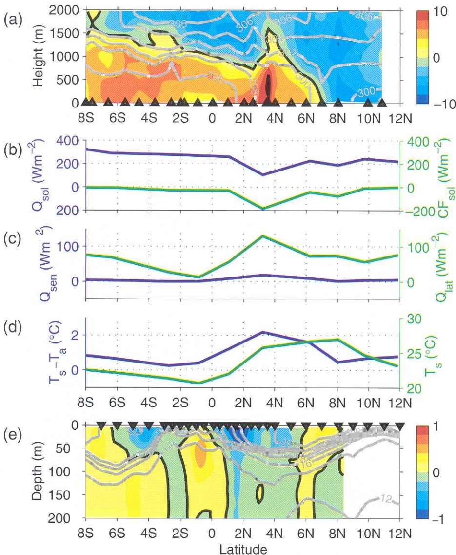
Fig. 2. Ocean and atmosphere fields along 95°W are shown as measured from the NOAA ship Ron Brown in November 1999. (a) Surface to 2000-m-height meridional winds (in units \text{ms}^{-1} , positive from the south, shaded intervals of 2 \text{ms}^{-1} ), and virtual potential temperature (in units ^{\circ}\text{K} , contour interval (CI) of 2^{\circ}\text{K} ). Triangles indicate locations of radiosonde launches. (b) Blue indicates incoming solar radiation and green indicates solar radiation cloud forcing (both in units \text{Wm}^{-2} ). (c) Sensible (blue) and latent (green) heat loss by the ocean are shown (both in units \text{Wm}^{-2} ). (d) Sea and air surface temperature difference (blue) and sea surface temperature (green) are also indicated (both in units ^{\circ}\text{C} ). (e) Surface to 200-m-depth zonal current (in units \text{ms}^{-1} , positive from west, shaded intervals of 0.2 \text{ms}^{-1} ), and potential temperature (in units ^{\circ}\text{C} , CI of 2^{\circ}\text{C} ) are shown. Inverted triangles indicate locations of CTD casts.
