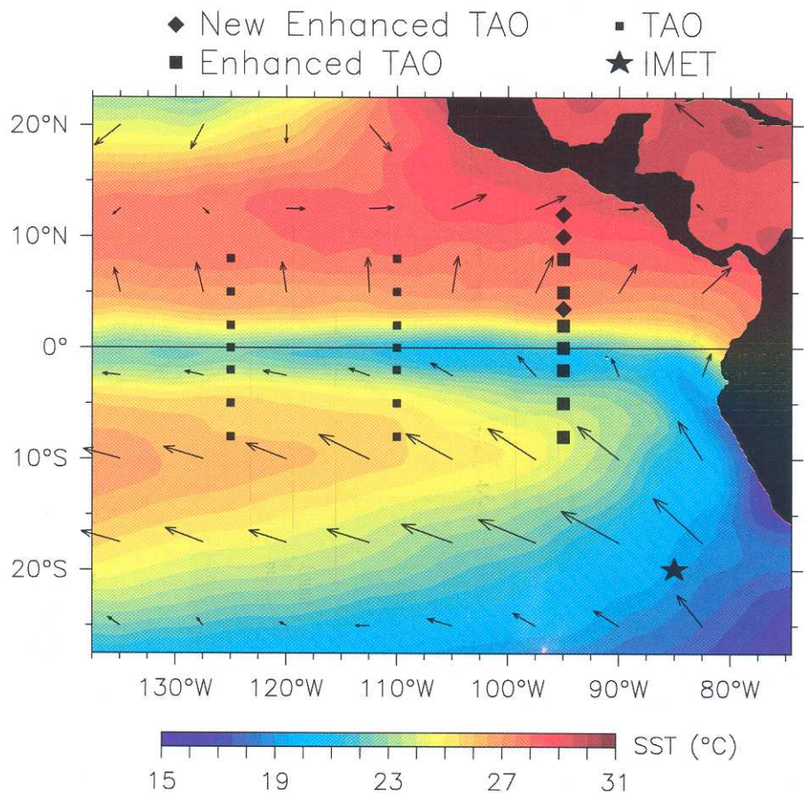
Fig. 1. The EPIC mooring array is shown in relation to the September 1998 composite SST and European Center for Medium-range Weather Forecasts wind fields.
