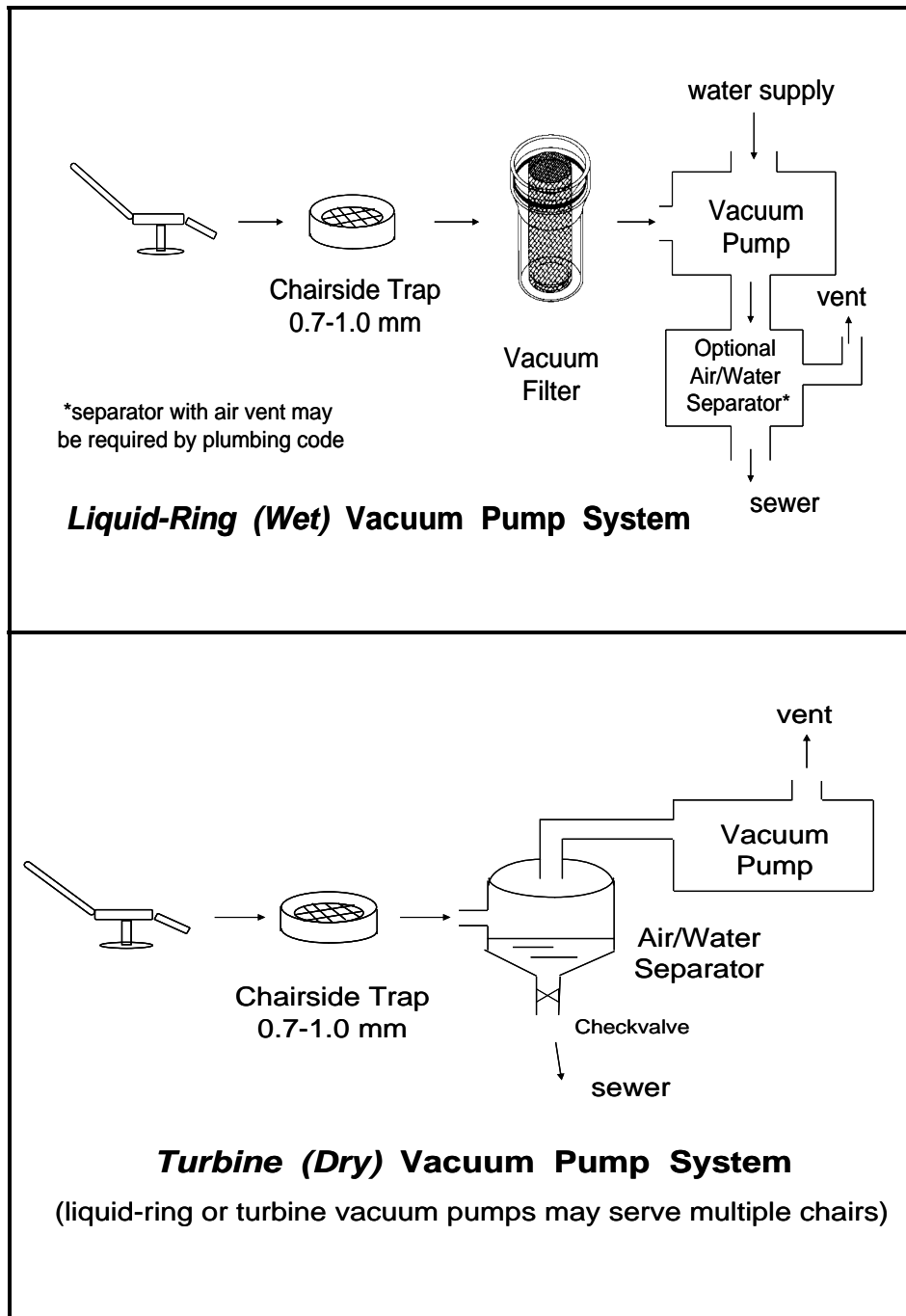
Figure 4 - Typical dental clinic waste flow systems (without amalgam separator)
