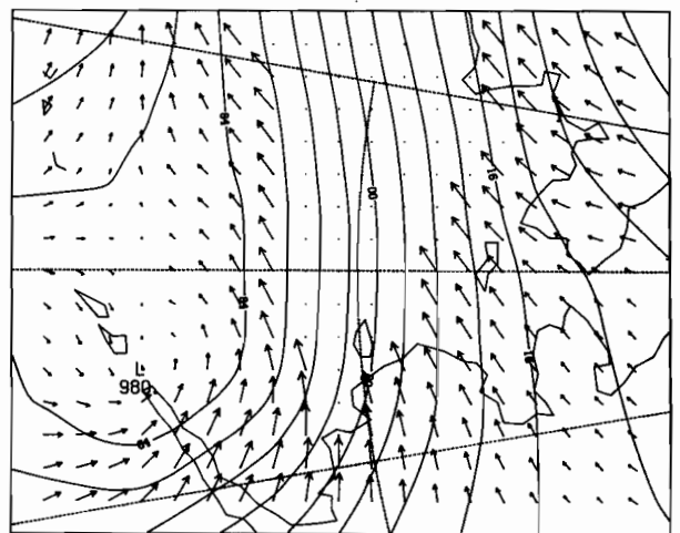
12Z 24 FEB 1981
