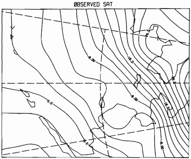
12Z 7 MAR 1981
