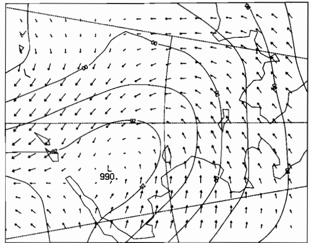
12Z 16 MAR 1981
