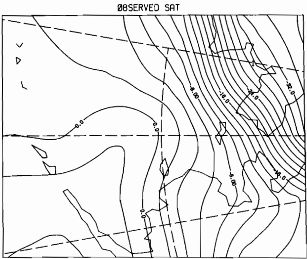
12Z 8 MAR 1981
