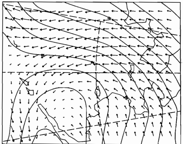
12Z 14 MAR 1981
