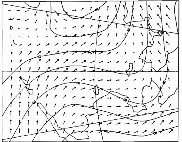
12Z 19 MAR 1981
