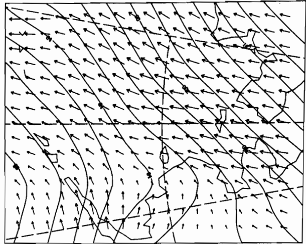
12Z 12 MAR 1981
