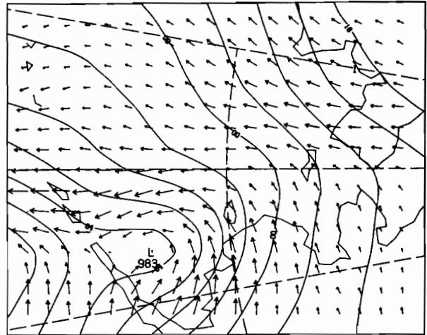
12Z 7 MAR 1981
