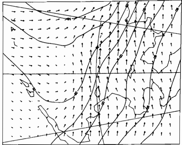
12Z 18 MAR 1981
