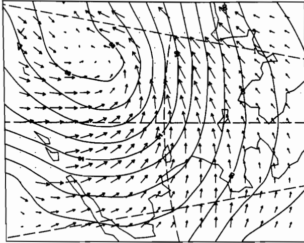
00Z 28 FEB 1981
