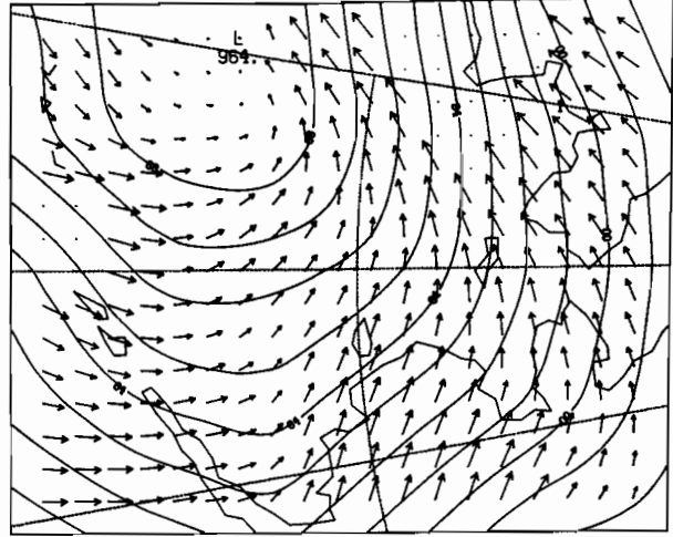
12Z 28 FEB 1981
