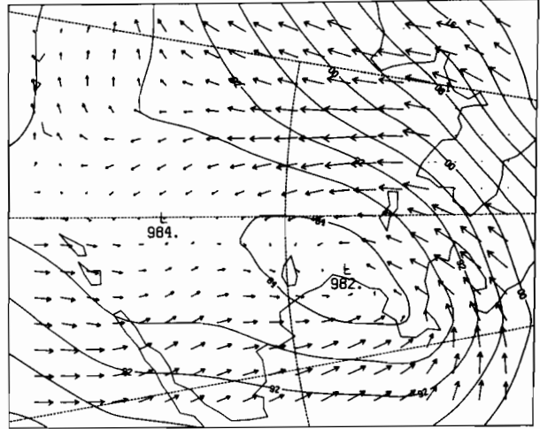
12Z 25 FEB 1981
