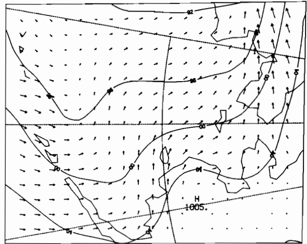
12Z 3 MAR 1981
