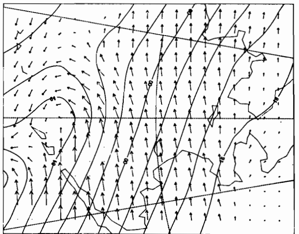
12Z 20 MAR 1981
