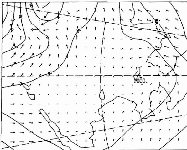
00Z 27 FEB 1981
