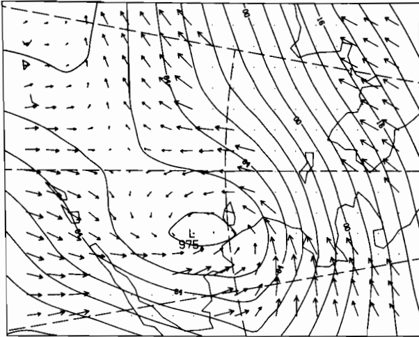
00Z 25 FEB 1981
