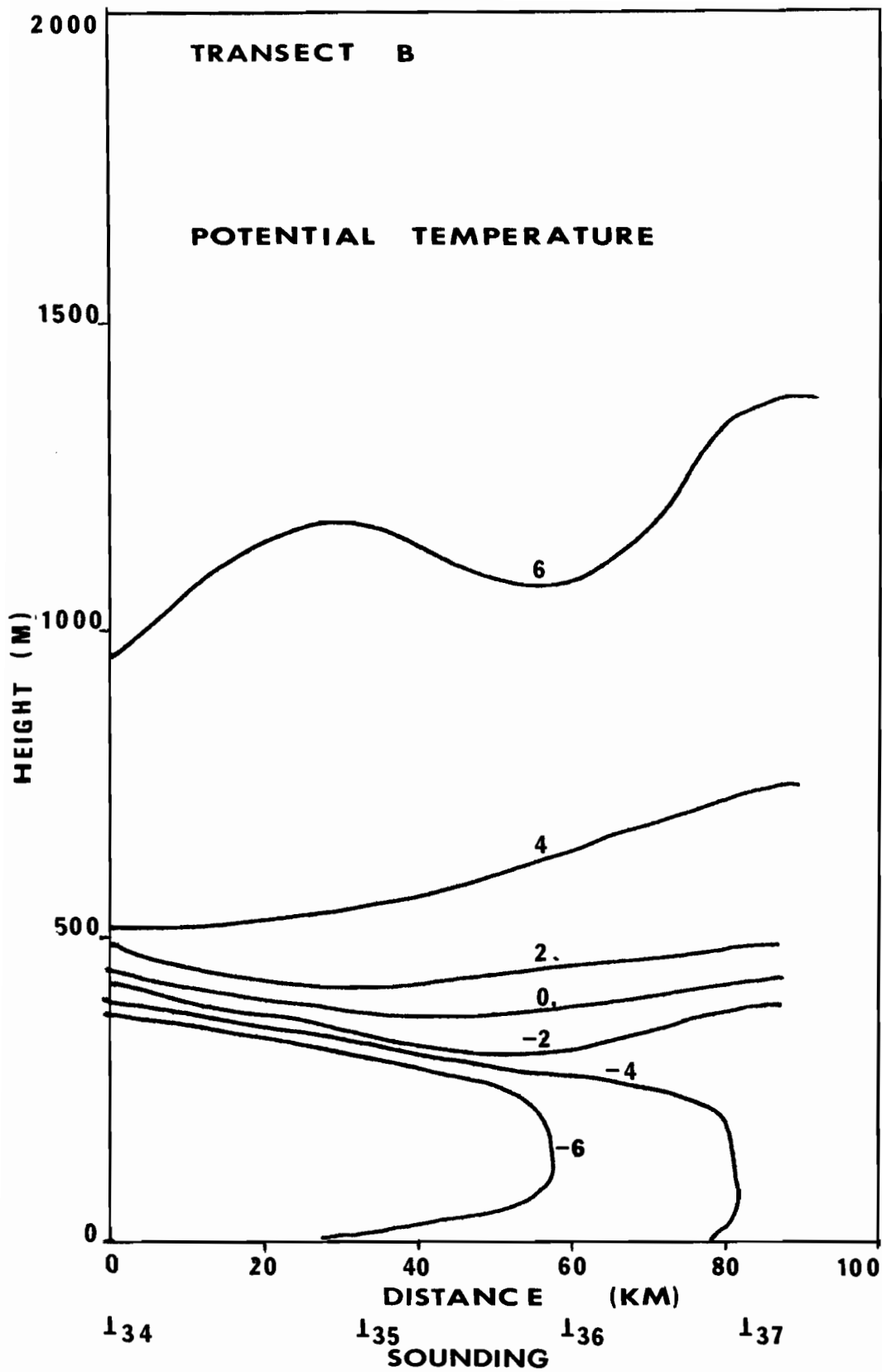
Figure 7.--Cross section of potential temperature for transect B.
