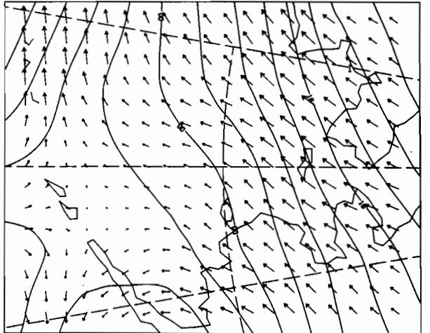
12Z 11 MAR 1981
