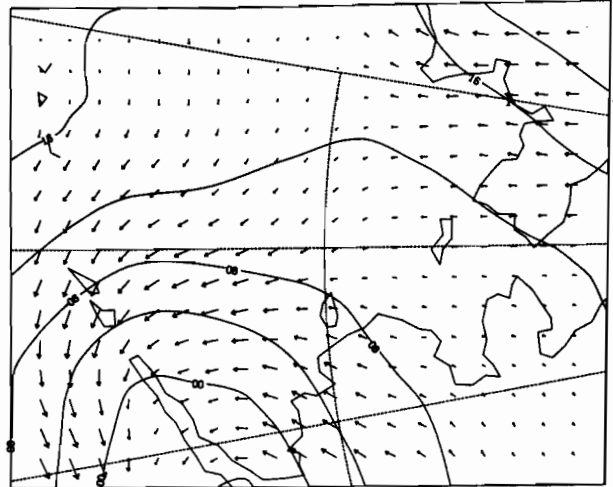
12Z 22 FEB 1981
