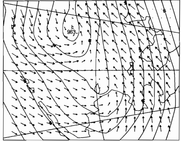
12Z 1 MAR 1981
