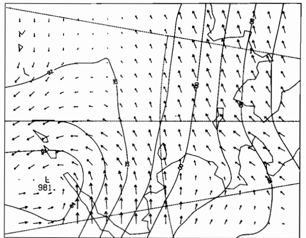
12Z 4 MAR 1981
