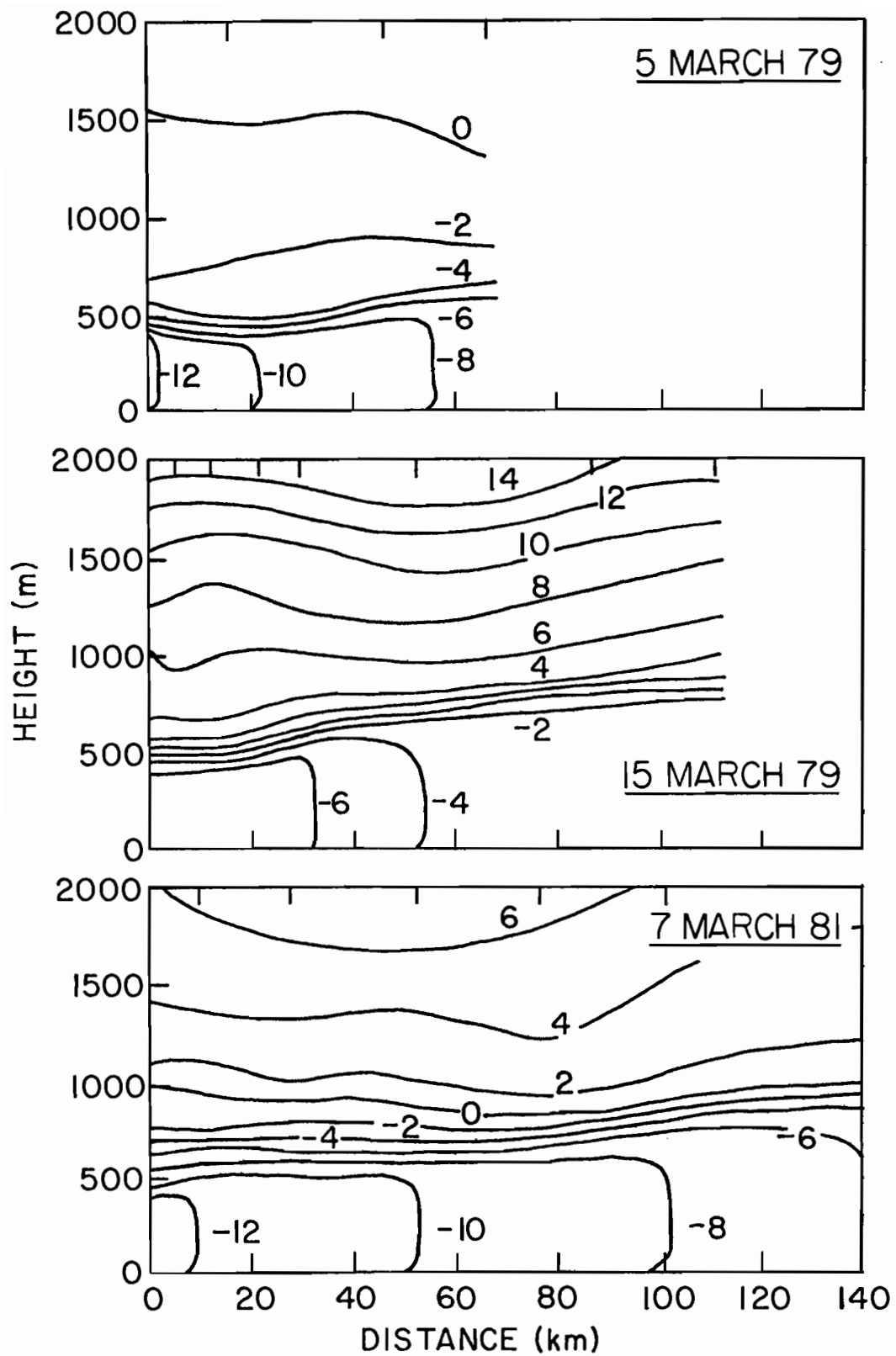
Figure 8.--Cross sections from 1979 and 1981 compared.
