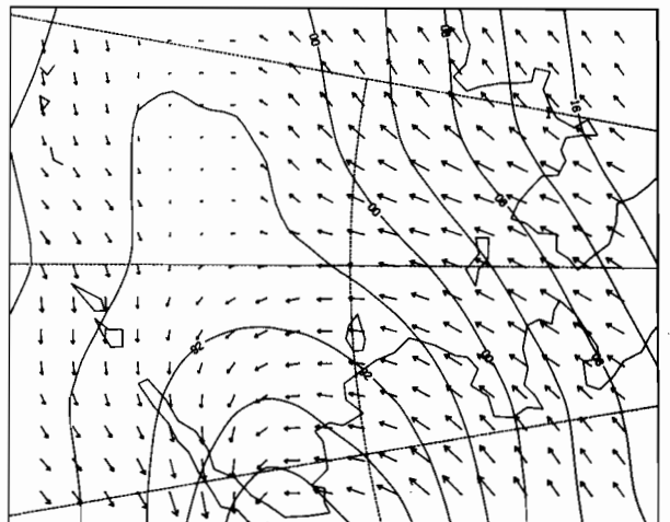
12Z 5 MAR 1981
