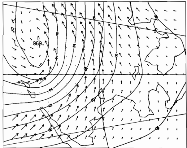
12Z 27 FEB 1981
