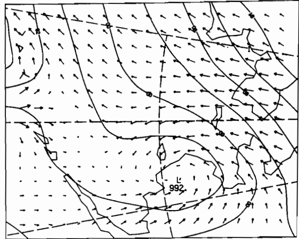
12Z 6 MAR 1981
