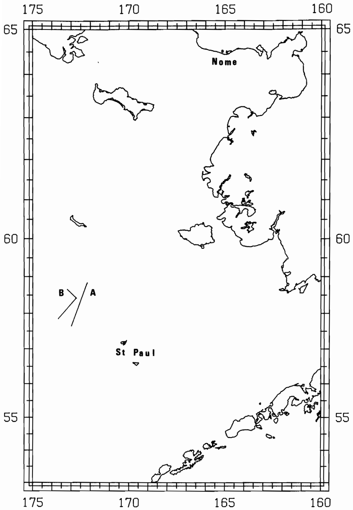
Figure 2.--Map of the Bering Sea with the position of the two transects.
