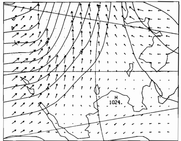
12Z 23 FEB 1981
