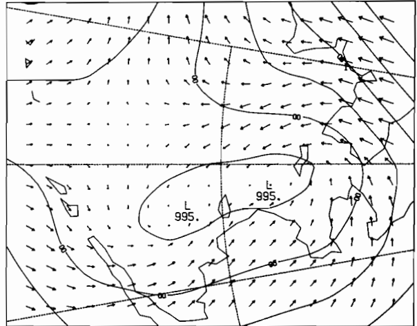
12Z 26 FEB 1981
