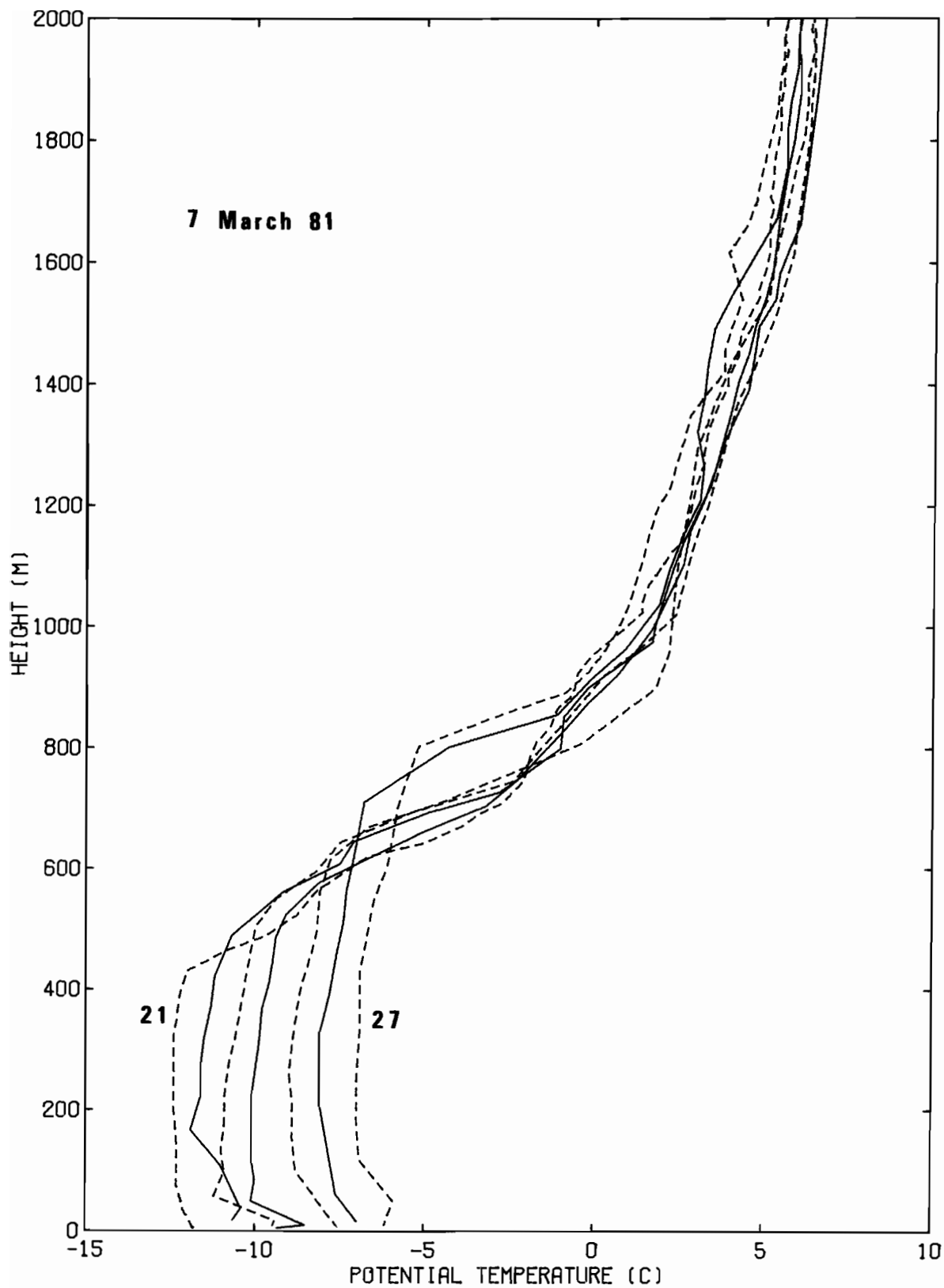
Figure 3.--Potential temperatures for transect A.
