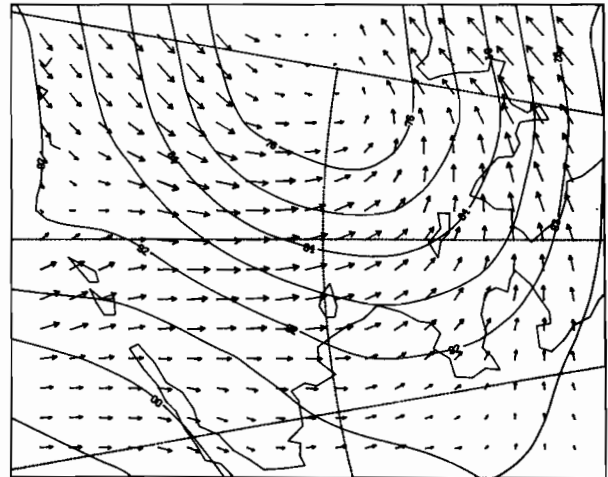
12Z 2 MAR 1981
