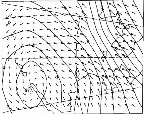
12Z 9 MAR 1981
