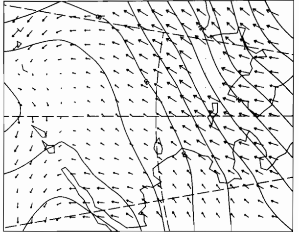
12Z 10 MAR 1981
