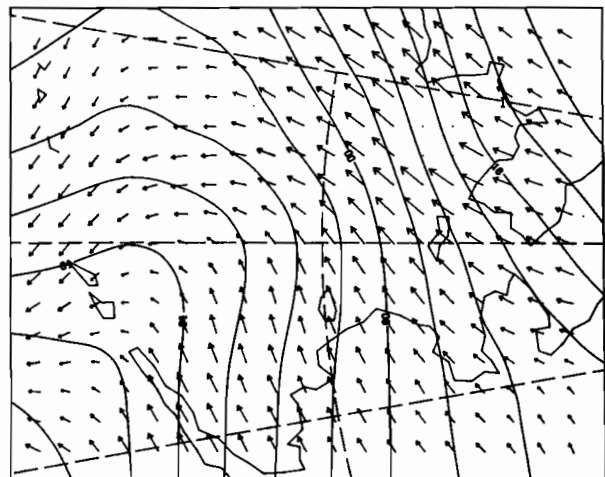
12Z 8 MAR 1981
