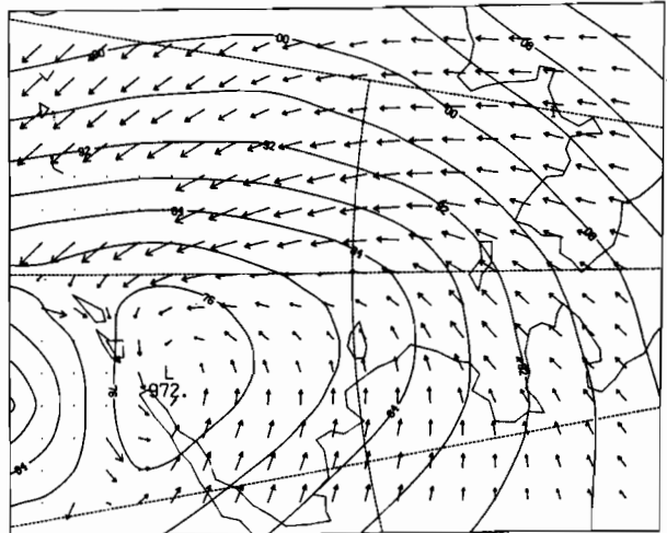
12Z 15 MAR 1981
