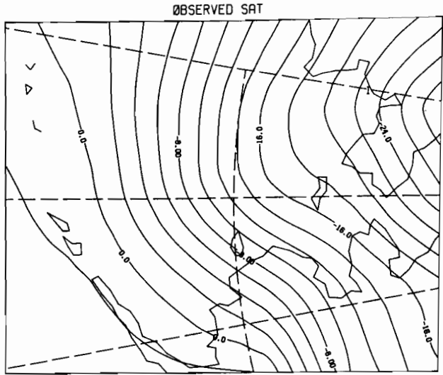
12Z 6 MAR 1981
