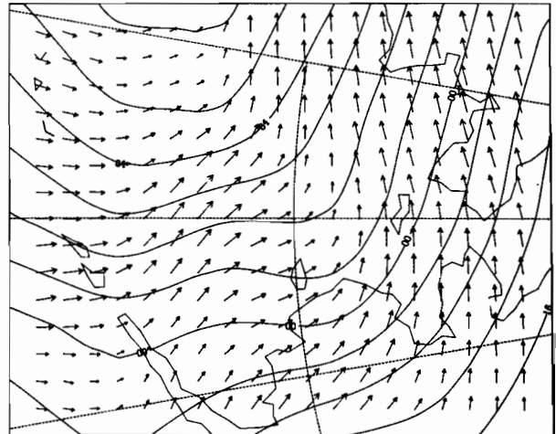
12Z 17 MAR 1981
