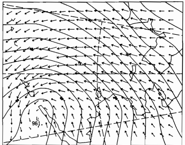
12Z 13 MAR 1981
