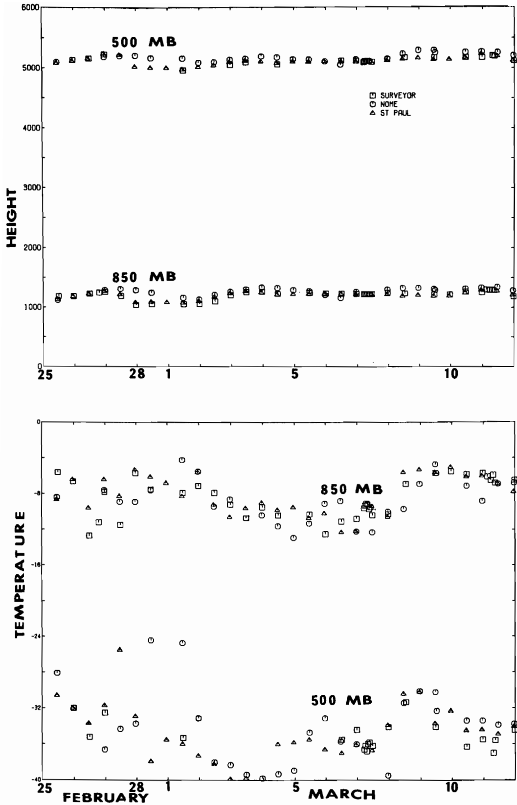
Figure 1.--850- and 500-mb heights and temperatures.
