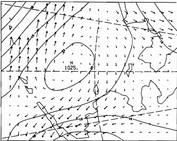
00Z 23 FEB 1981
