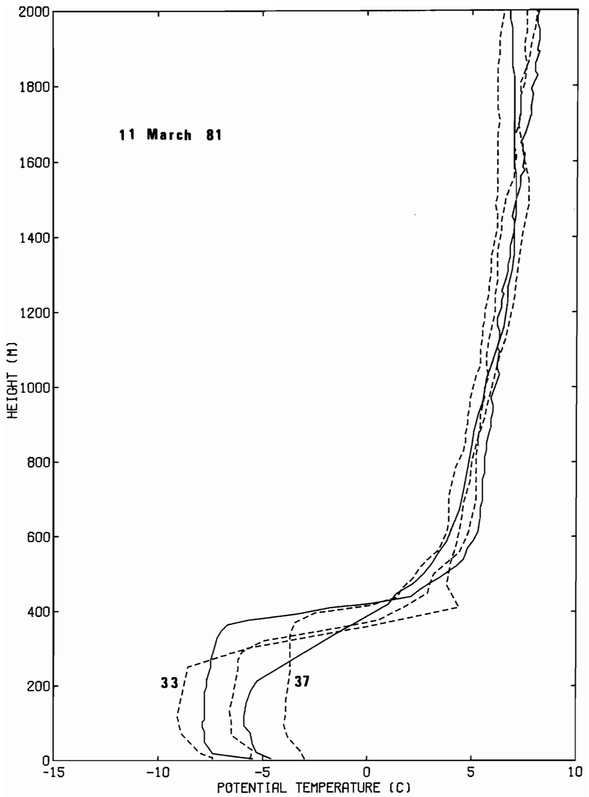
Figure 6.--Potential temperature for transect B.
