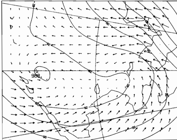
00Z 26 FEB 1981
