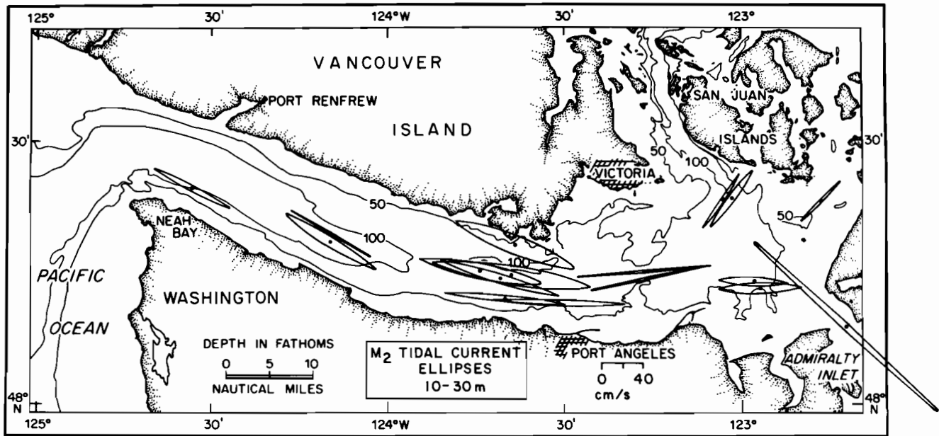
Figure 20.-- M_2 tidal current ellipses at 10- to 30-m depth.
