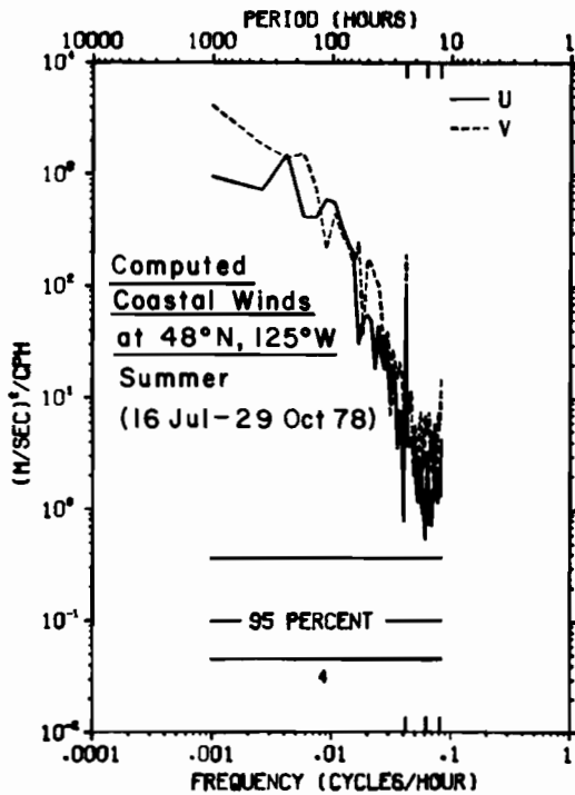
Figure 11.--Density spectra of east-west (U, —) and north-south (V, ---) wind spectra at 48°N, 125°W, computed by Bakun (1977) and at Race Rocks during winter and summer conditions.
