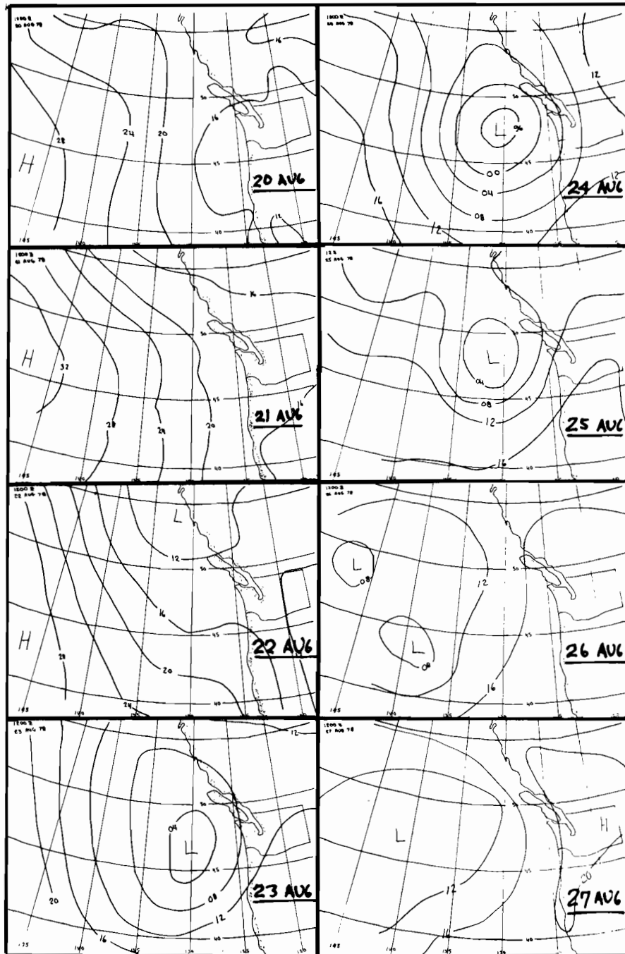
Figure 31.--Surface pressure maps showing stationary low pressure system centered 300-400 km off the Washington coast between 23 and 25 August 1978.
