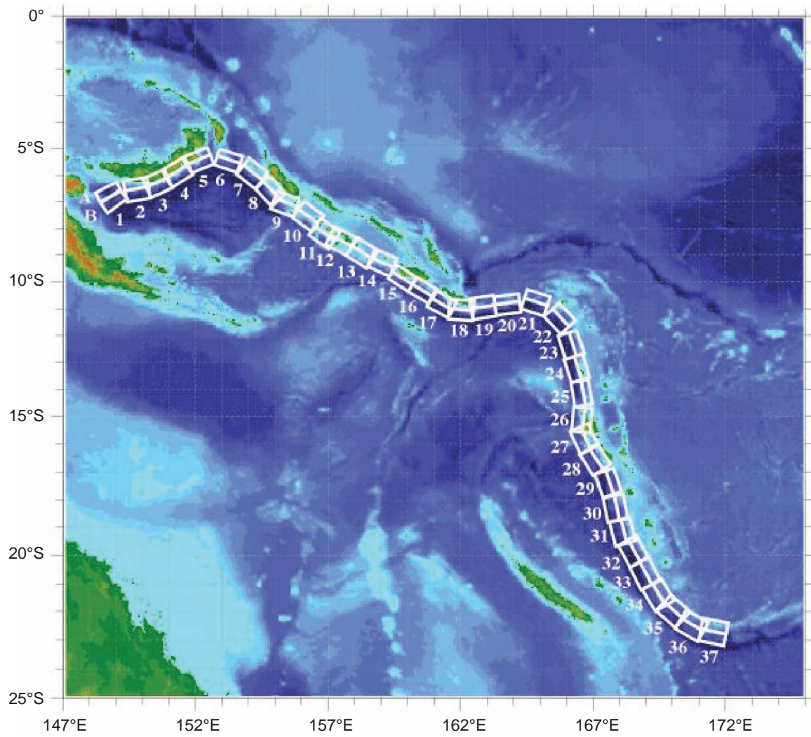
Figure B7: New Britain-Solomons-Vanuatu Subduction Zone unit sources.
