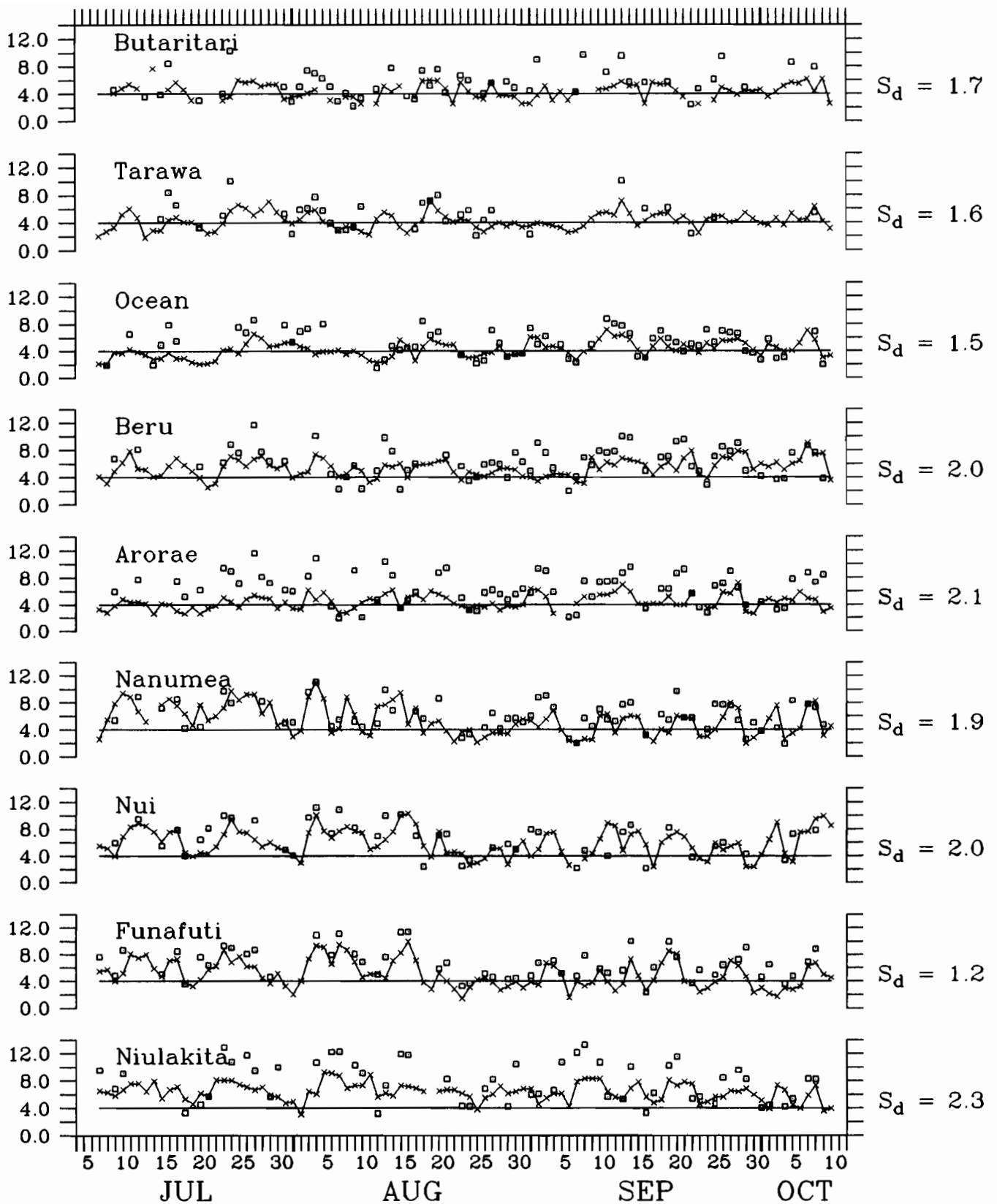
Figure 7. Speed ( \text{m s}^{-1} ) of daily average winds at the nine islands, and SASS-1. The standard deviation of the daily average speed difference ( S_d , SASS-1 minus island) is given at the right for each island.
