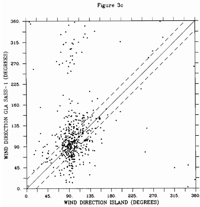
Figure 3. Scatter plots of island observations and SASS. (a) Wind speed, island and SASS-1. (b) Wind speed, island and SASS-2. (c) Wind direction, island and GLA SASS-1. (d) Wind direction, island and CDA SASS-1.
