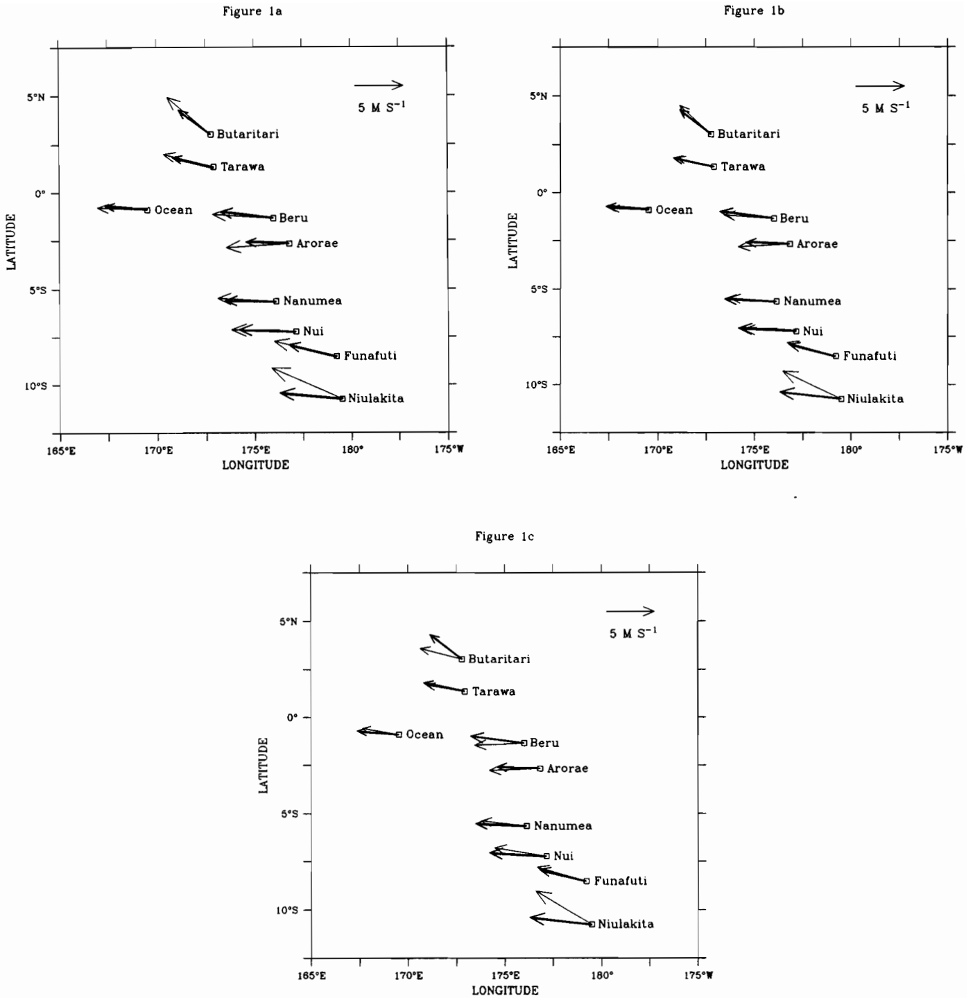
Figure 1. Complete-mission vector average winds, island observations (dark vectors) compared with SASS (light). (a) CDA SASS-1. (b) CDA SASS-2. (c) GLA SASS-2.
