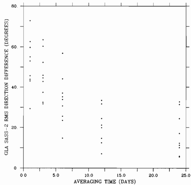
Figure 4. RMS differences between island observations and GLA SASS-2 as a function of averaging time. (a) Speed. (b) Direction.
