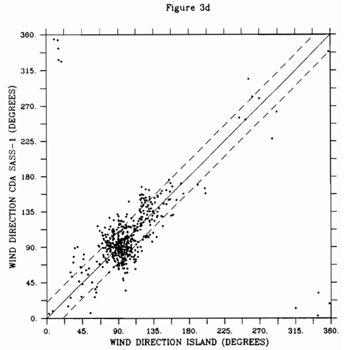
Figure 3. Scatter plots of island observations and SASS. (a) Wind speed, island and SASS-1. (b) Wind speed, island and SASS-2. (c) Wind direction, island and GLA SASS-1. (d) Wind direction, island and CDA SASS-1.
