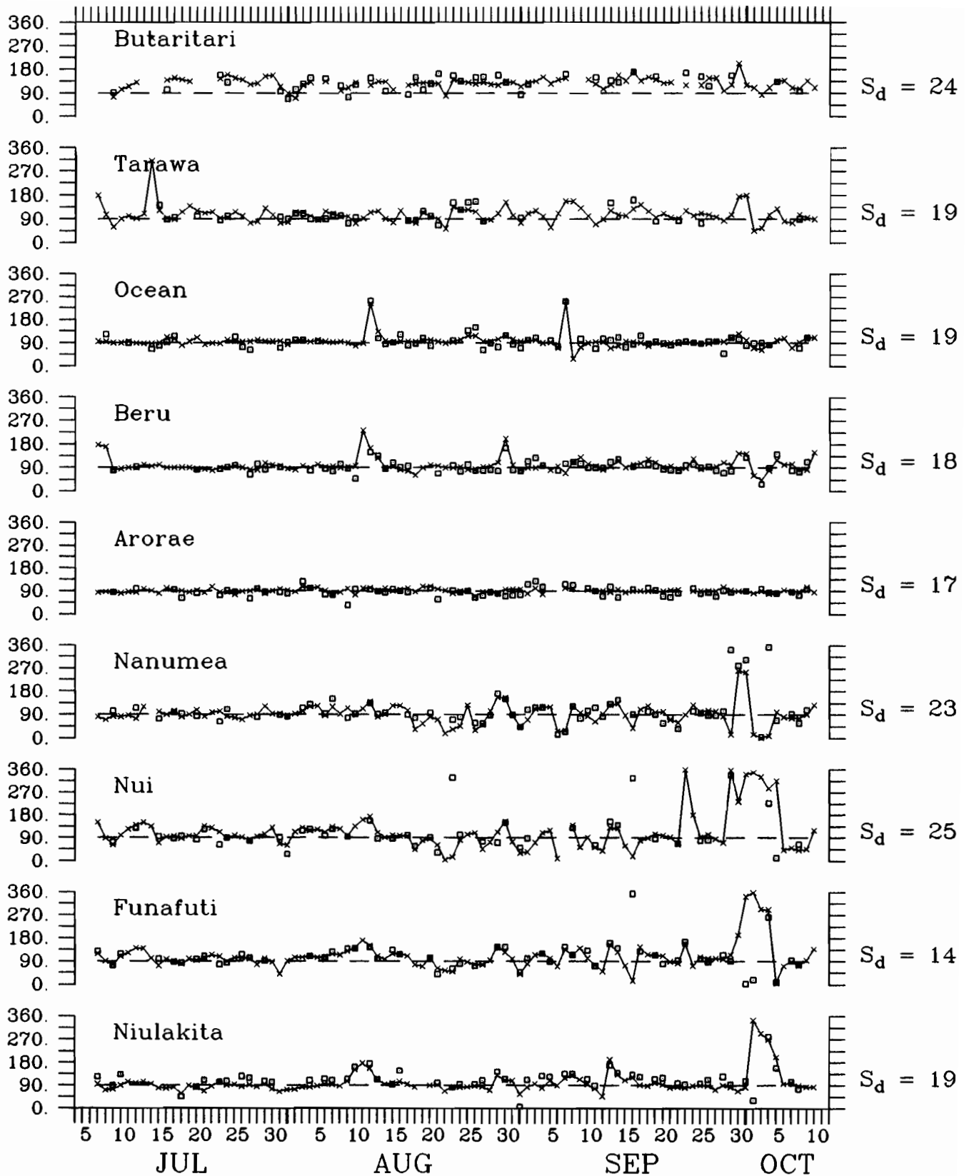
Figure 6. Direction (degrees) of daily average winds at the nine islands, and CDA SASS-1. The standard deviation of the daily average direction difference ( S_d , CDA minus island) is given at the right for each island.
