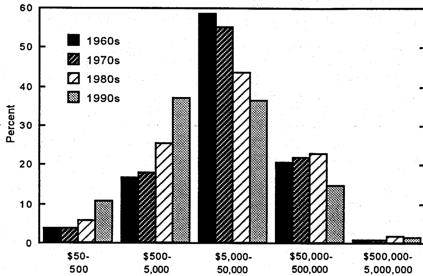
FIGURE 41. Decadal changes in US lightning damage reports for the five most frequent cost categories.
