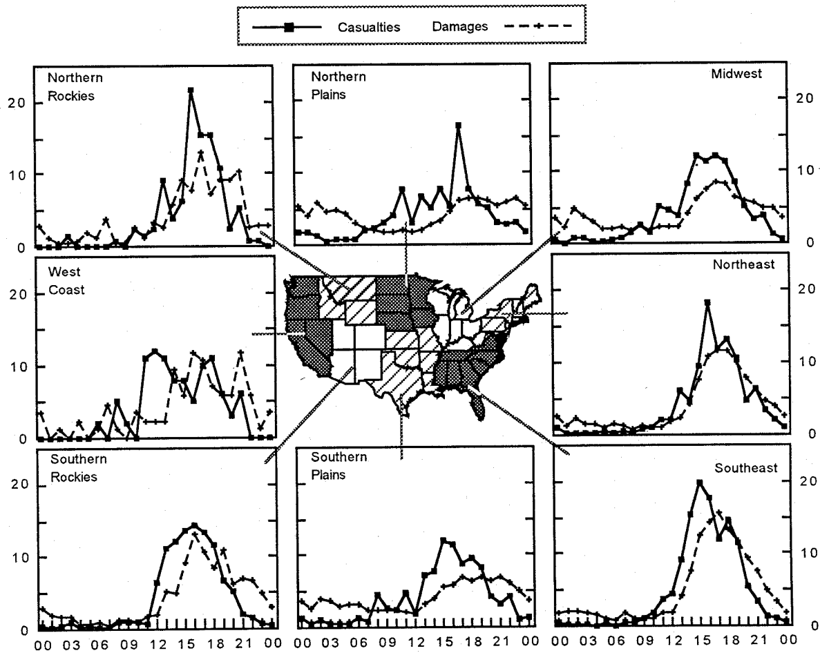
FIGURE 32. Time of day of lightning casualties (solid line) and damage reports (dashed) by region in %.
