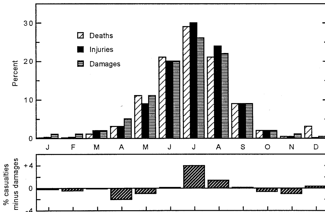
FIGURE 26. Top: Monthly variations of lightning fatalities, injuries, and damage reports for the US from 1959 to 1994. Bottom: Percent casualties minus damage reports by month.
