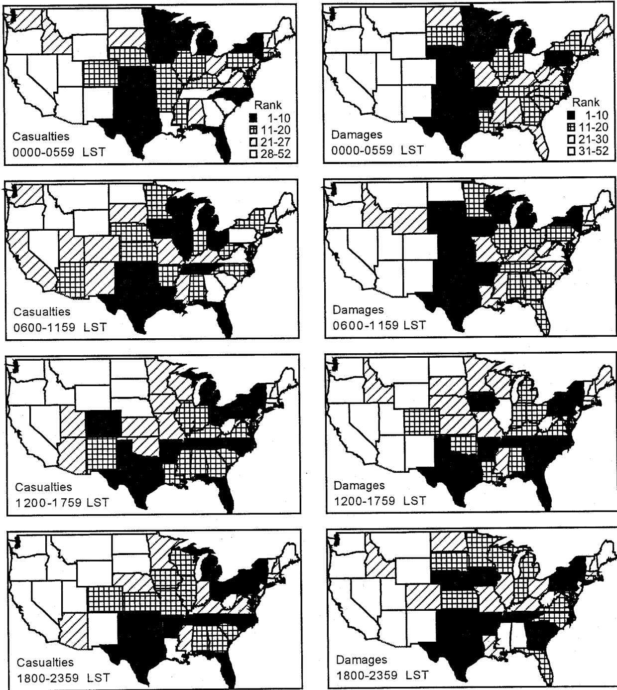
FIGURE 33. Rank of lightning casualties and damage reports by 6-hour periods and state of the US from 1959 to 1994.
