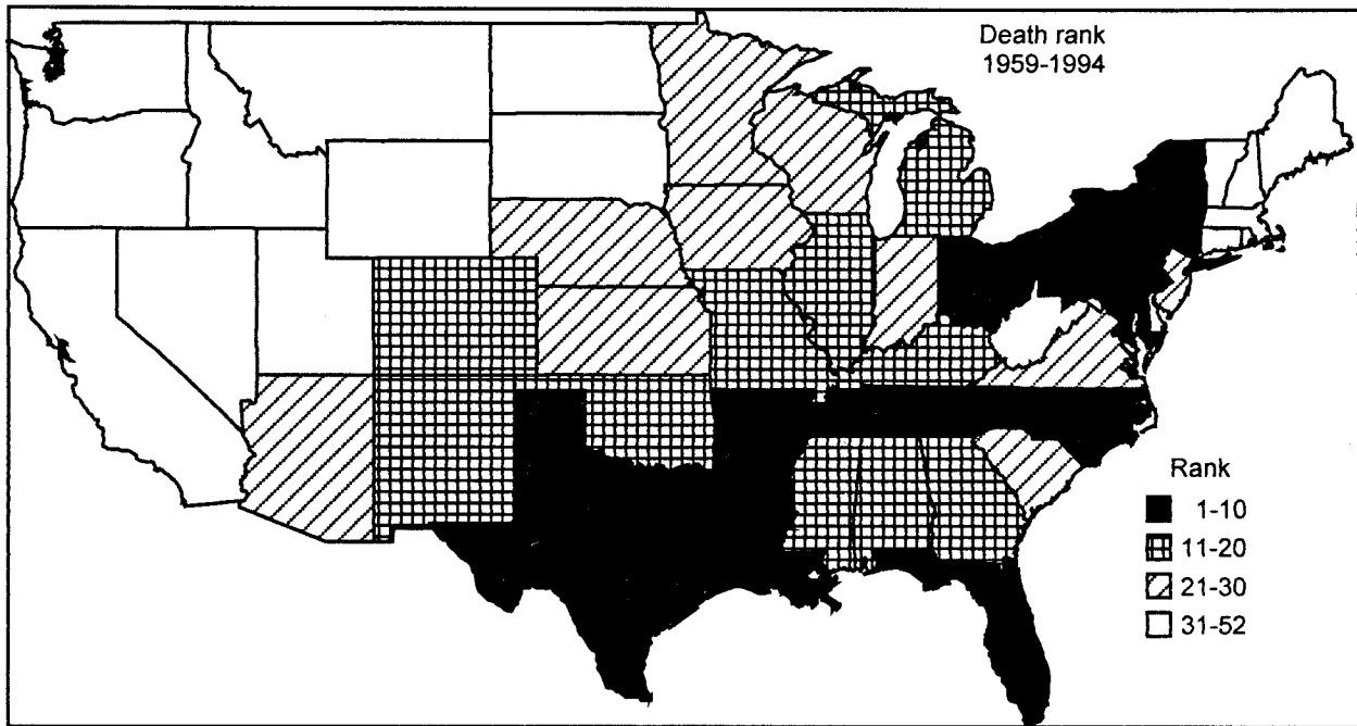
FIGURE 5. US map of lightning deaths ranked by state from 1959 to 1994.
