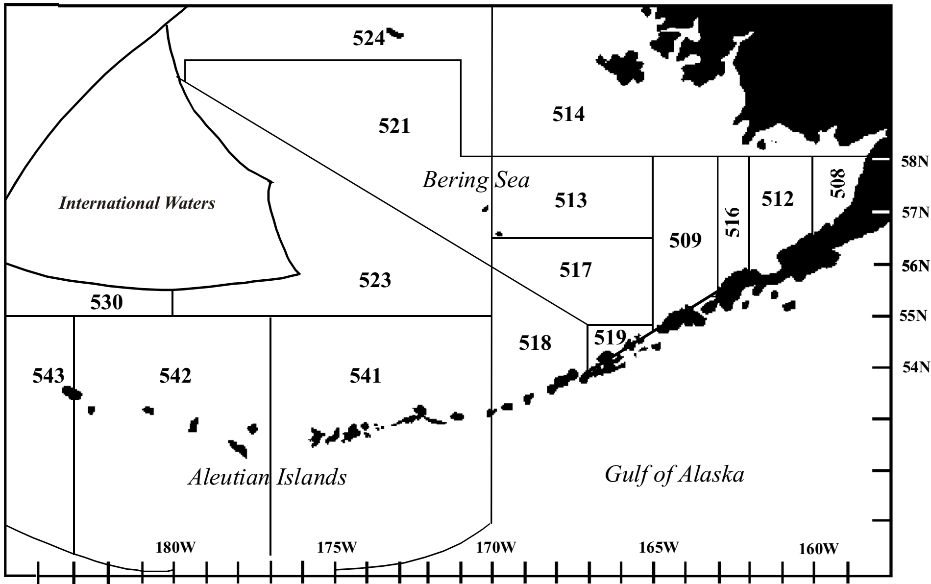
Figure 1.2-2. Bering Sea and Aleutian Islands sub-areas of management and reporting.
