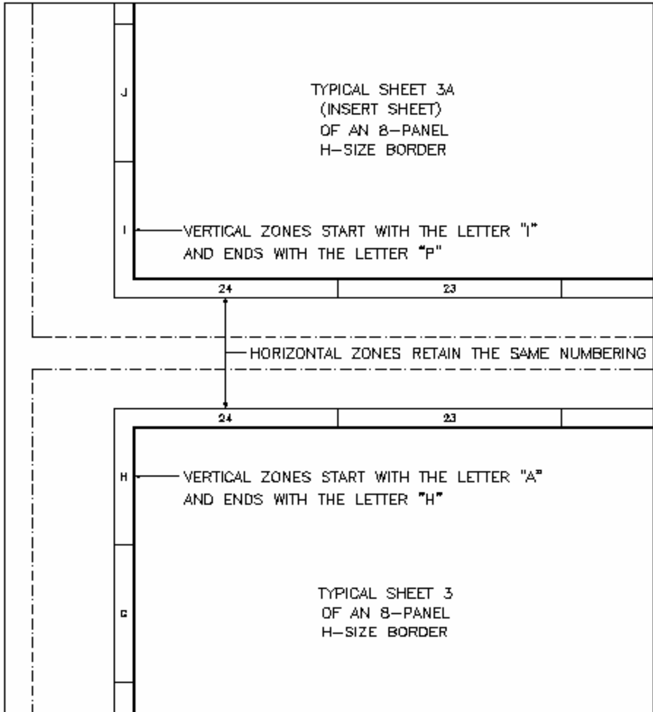
FIGURE 5-1 DRAWING ZONES FOR INSERT SHEETS
