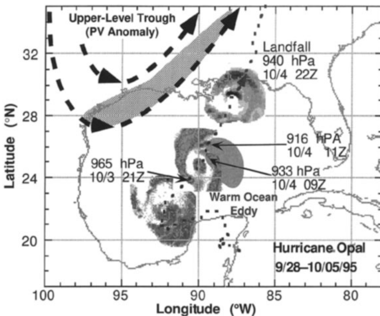
FIG. 1. Track of Hurricane Opal from 28 September to 5 October 1995. The storm track is drawn as a bold dotted line. The upper-level trough location at 1200 UTC 4 October derived from upper-level analyses is denoted by the bold dashed line and the positive PV anomaly associated with the trough by the light stippling. The warm core ocean eddy location derived from TOPEX altimeter data is depicted by the dark stippling. The storm's internal structure is represented by SSM/I 85-GHz imagery at 1629 UTC 3 October, 0337 UTC 4 October, and 1555 UTC 4 October. The 85-GHz blackbody temperatures are depicted as shades of gray; the darker shades denoting cooler temperatures and, therefore, precipitation size particles. The SSM/I data was provided by J. Hawkins (Naval Research Laboratory/Monterey), and the TOPEX/POSEIDON imagery used to find the location of the warm core eddy was provided by G. Goni (Remote Sensing Group, University of Miami/Rosenstiel School for Marine and Atmospheric Sciences).
