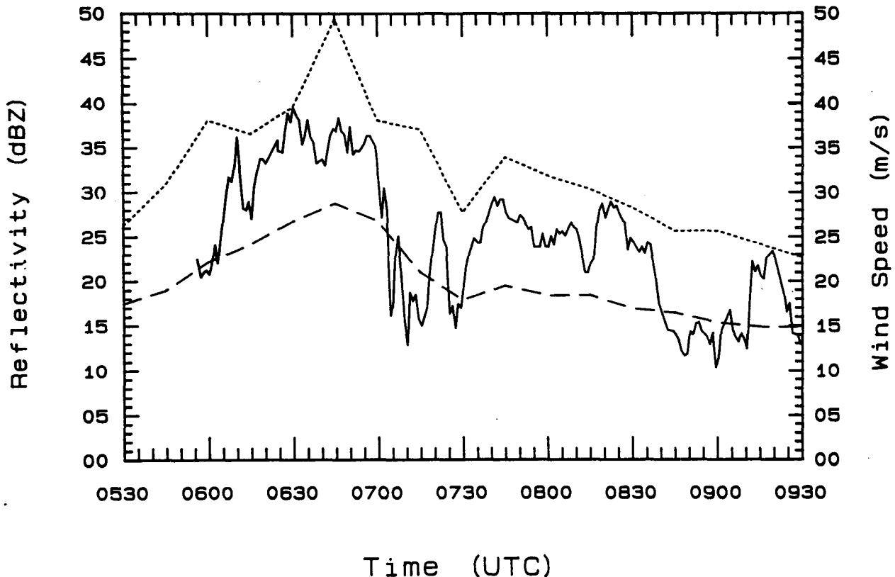
FIG. 11. Time series of radar reflectivity (solid line) for the location of Shaw Air Force Base as measured by the Charleston NWS radar. Peak gusts and 15-min mean winds (dashed lines) are from the Shaw Air Force Base anemometer trace from 0530–0930 UTC on 22 September 1989.
