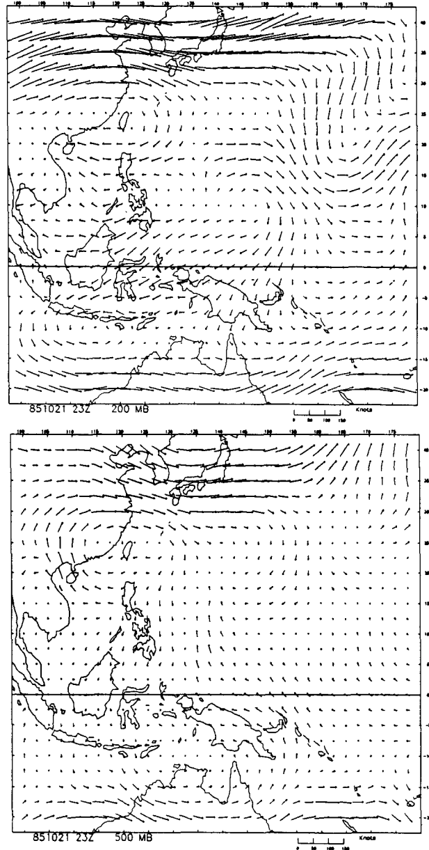
FIG. 23. An example of the 200- and 500-mb BMRC objective analysis wind fields.
