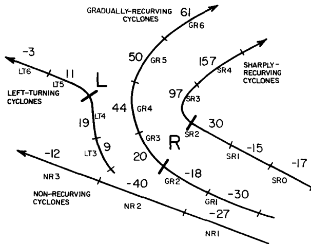
FIG. 22. The RN values for the sharply recurving, gradually recurving, left-turning, and nonrecurving cyclone time periods.
