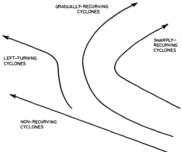
FIG. 4. Typical tracks for the four basic types of cyclones defined and analyzed in this study.
