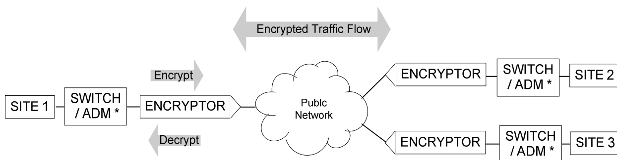
Figure 1. Encryptor Operation.
