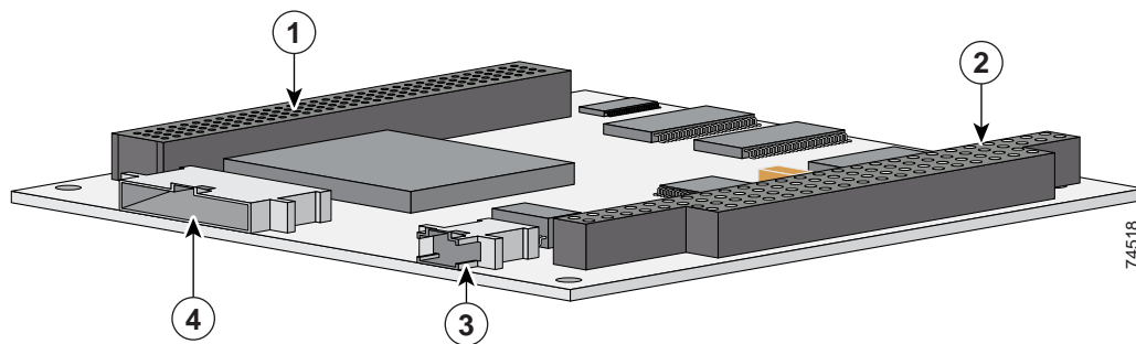
Figure 1 The Cisco 3200 Mobile Access Router Card
