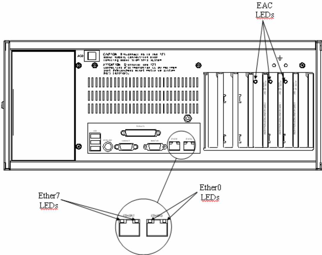
Figure 13 - Brick 1100 Rear Panel LEDs
