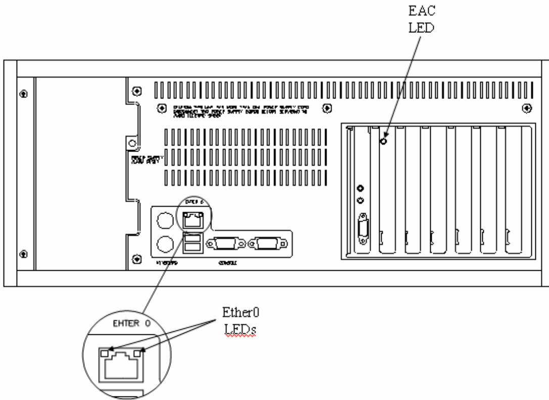
Figure 12 - Brick 1000 Rear Panel LEDs
