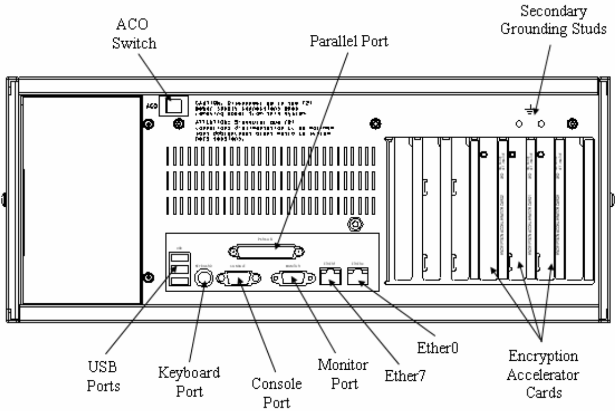
Figure 7 - Brick 1100 Physical Interfaces
