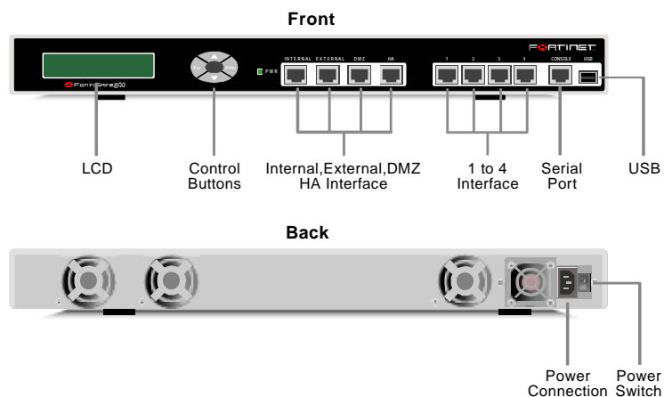
Figure 4: FortiGate-800 Front and Rear Panels
