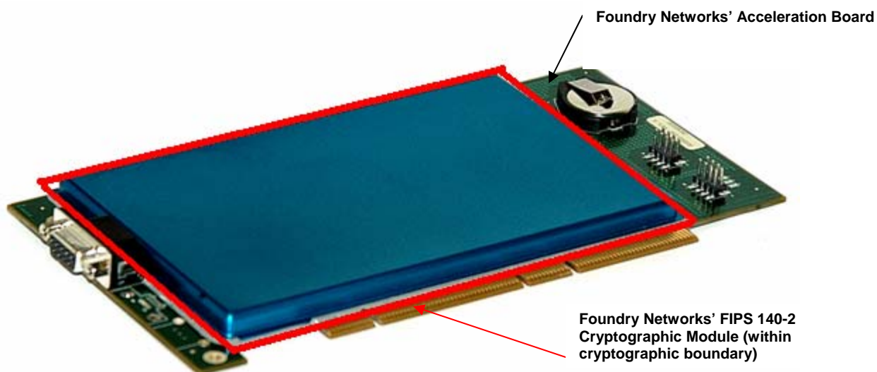
Figure 2-1. Foundry Networks' FIPS 140-2 Cryptographic Module, Level 2
