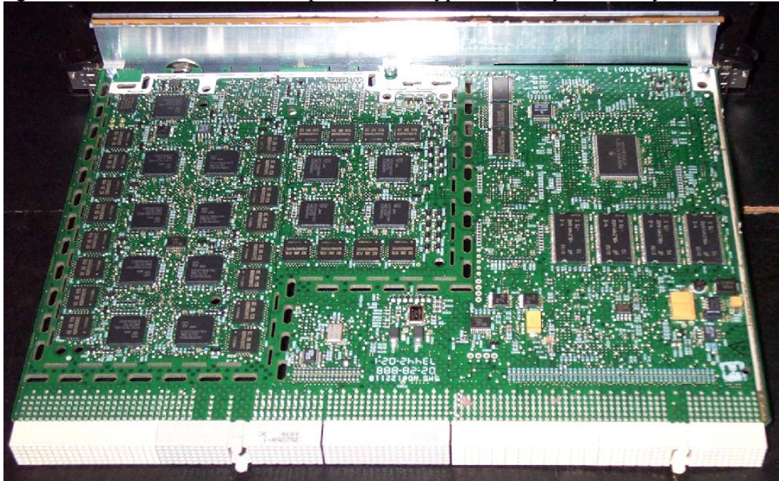
Figure 2: MGE SC back w/o tamper shield. Crypto boundary defined by dashed 'line'.
