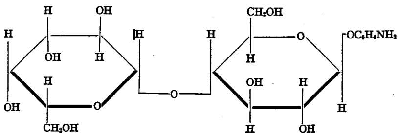
p -Aminophenol \beta -lactoside
