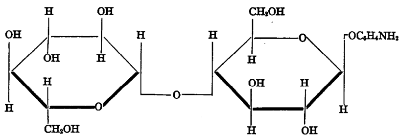
p -Aminophenol \beta -cellobioside
