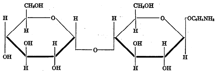
p -Aminophenol \beta -maltoside
