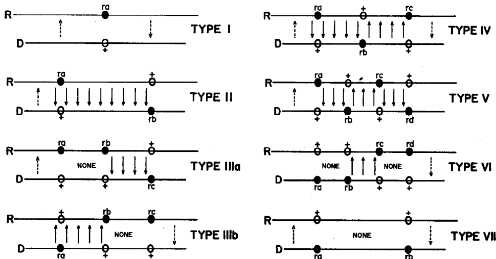
FIGURE 2.—Diagram of the seven kinds of transformation crosses. R = recipient nucleotide sequence; D = donor nucleotide sequence; ● = mutated site; ○ = +++ site; a solid arrow indicates location of a restricted exchange event and a dashed arrow indicates location of an unrestricted exchange event. TYPE I. One-factor cross. In order to recover a +++ recombinant, two unrestricted exchange events must occur, one on either side of the recipient site which must be eliminated from the recombinant chromosome. TYPE II. Two-factor trans cross. Recovery of a +++ recombinant is dependent upon the occurrence of a restricted exchange event in the interval between the recipient and donor sites, as well as the occurrence of an unrestricted exchange event outside this interval. TYPE III (a and b). Three-factor cross. Recovery of a +++ recombinant depends upon the occurrence of a restricted exchange event in one interval and the absence of an odd number of exchange events in a contiguous interval. The position of the single unrestricted exchange event is unspecified. TYPE IV. Three-factor cross. Two restricted exchange events, one in each of two adjacent intervals, and two unrestricted exchange events are required in order to recover a +++ recombinant. TYPE V. Four-factor cross. Recovery of a +++ recombinant is dependent upon the occurrence of a restricted exchange event in each of three contiguous intervals, as well as the occurrence of a single unrestricted exchange event. TYPE VI. Four-factor cross. One unrestricted exchange event whose position is largely unspecified and one restricted exchange event in the interval rb to rc are required in order to recover a +++ recombinant. TYPE VII. Two-factor cis cross. Recovery of double transformant ( ra rb ) is dependent upon the occurrence of two unrestricted exchange events, accompanied by no or an even number of exchange events in the interval separating the two recipient sites.
