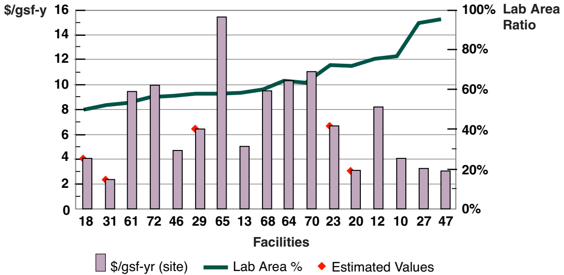
Figure 4. Normalized annual energy costs in laboratories (facilities with >50% of total floor area in labs).
