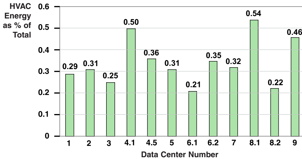
Figure 3. Heating, ventilating, and air-conditioning costs can vary from about 20% to 55% of total energy costs in datacenters, a sign of hidden inefficiencies.
