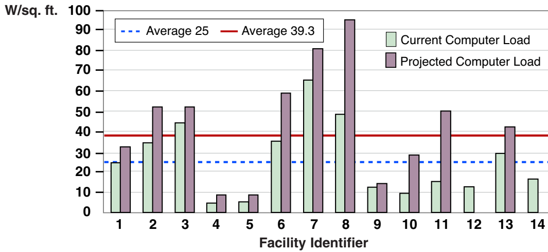
Figure 2. Bars show total power requirement per unit floor area for as-is conditions and if server racks were fully loaded.
