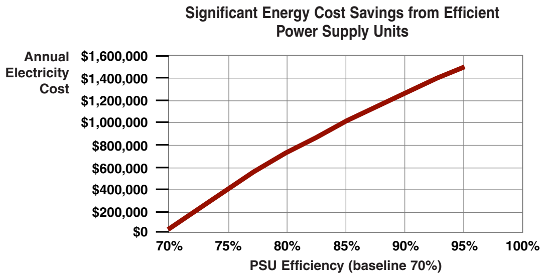
Figure 6. Savings potential in a typical data center. Energy-efficient server power supply units (PSUs).
