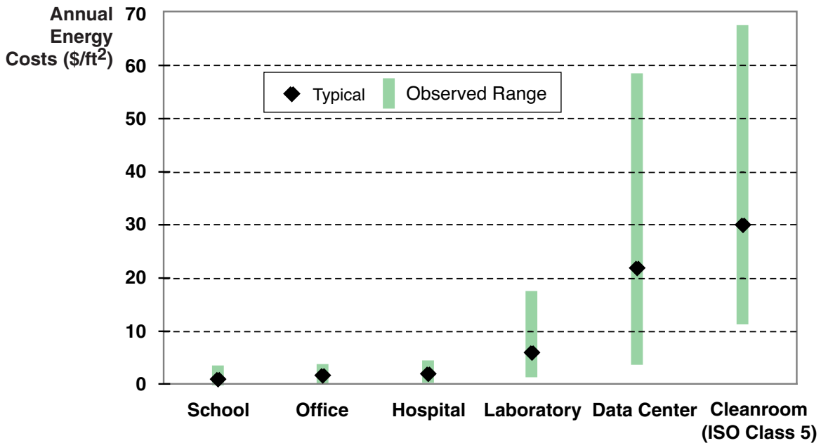
Figure 1. Data on schools, offices, and hospitals from USDOE/EIA Commercial Buildings Energy Consumption Survey (1999 values). High-Tech buildings from LBNL benchmarking databases ( http://hightech.lbl.gov ). Cleanrooms with the highest cleanliness standards can use significantly more energy than those shown.
