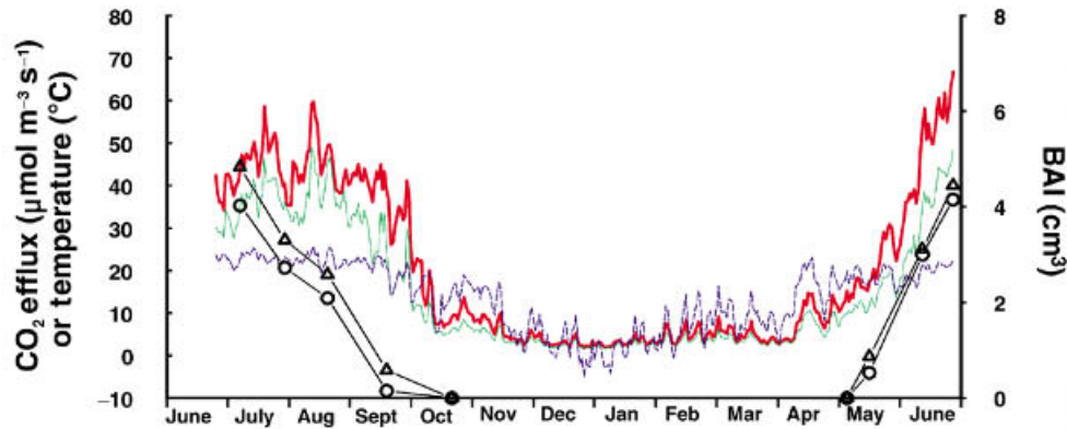
Fig. 1 Daily mean stem respiration rates in CO 2 -enriched sweetgum ( Liquidambar styraciflua ) trees (red line), control trees (green line), and stem temperatures (blue line) between June 2000 and June 2001. The means ( n = 2 ) were calculated from measurements taken at 112 min intervals on each of 6 trees in 2 plots of each treatment or in the case of power failure or equipment problems, rates were calculated using Q_{10} values and base rates. Basal area increments (BAI) of CO 2 -enriched trees (triangles) and control trees (circles) are also shown. BAI values are treatment means of the six 'respiration' trees in each plot. The BAI standard errors are not plotted but ranged from 7 to 14% of the means in the CO 2 -enriched trees, and from 13 to 28% of the means in the control trees ( n = 2 ).
