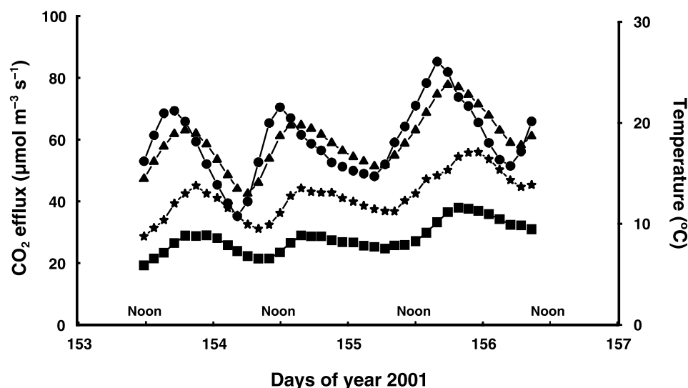
Fig. 3 Diurnal cycles of air and sweetgum ( Liquidambar styraciflua ) stem temperature and stem respiration by treatment ( n = 2 ) are shown for a period between June 2 and June 5, 2001. Circles, air temperature; triangles, stem temperature; stars, respiration (high CO 2 ); squares, respiration (control).
