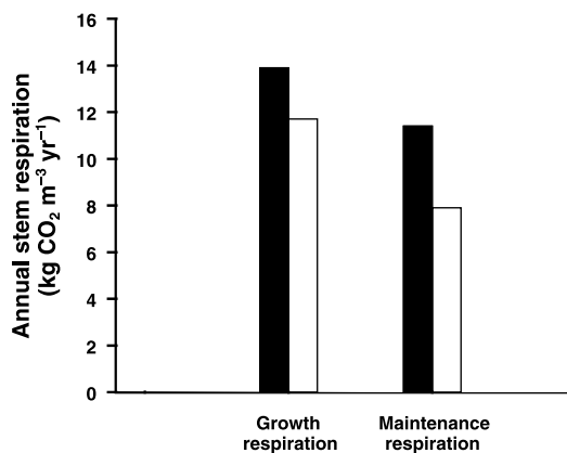
Fig. 2 Annual total stem growth respiration ( R_g ) and annual total stem maintenance ( R_m ) of sweetgum ( Liquidambar styraciflua ) trees. Annual total R_m = dormant season R_m plus growing season R_m . Dormant season R_m was calculated by summing measured dormant season daily average respiration rates. Growing season R_m was calculated from Q_{10} values and base rates at 10°C ( R_{10} ) determined during the dormant season measurements. Annual total R_g = annual total respiration (sums of measured daily average respiration rates minus predicted R_m ). Closed columns, high CO 2 ; open columns, control.
