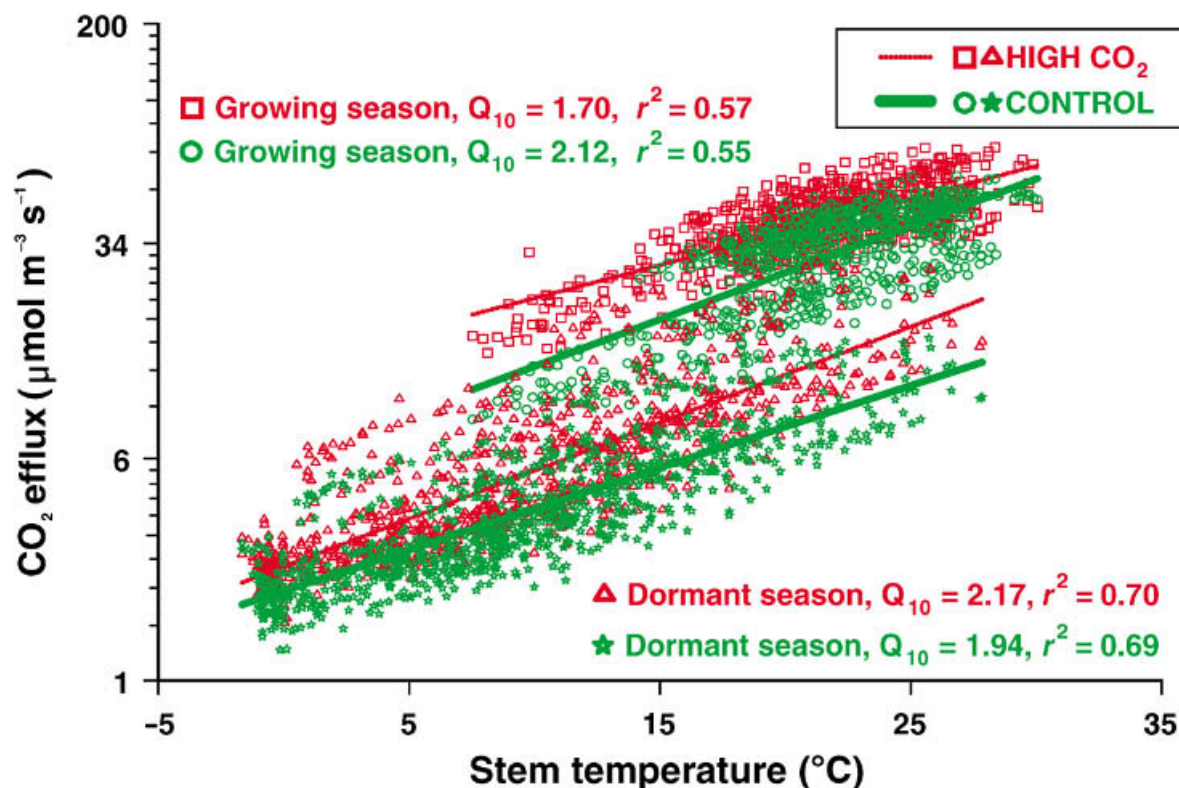
Fig. 4 Measured (at 112-min intervals) treatment average ( n = 2 ) stem respiration plotted against stem temperature of sweetgum ( Liquidambar styraciflua ). Dormant season and growing season data are plotted separately. The Q_{10} values and R_{10} rates were calculated for each season and each treatment from the regression lines shown for each set of data.
