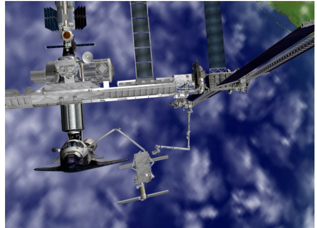
The P6 truss is handed between the station's robotic arm and the shuttle's robotic arm during its installation.
