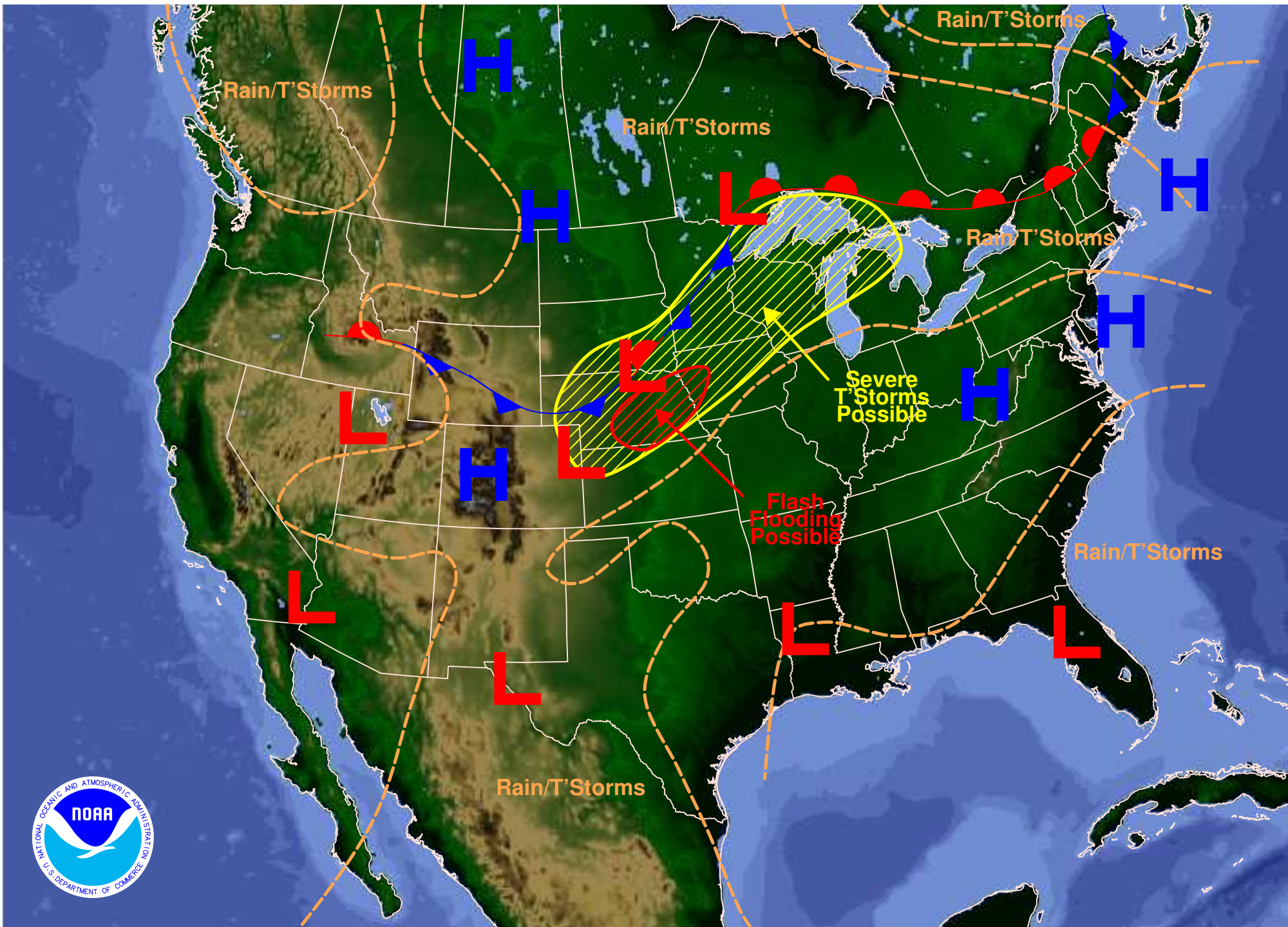
Weather Forecast for Thursday, July 17, 2008 DOC/NOAA/NWS/NCEP/Hydrometeorological Prediction Center Prepared by Engelman based on HPC, SPC, and TPC forecasts.
