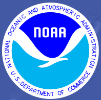
Weather Forecast for Friday, May 23, 2008 DOC/NOAA/NWS/NCEP/Hydrometeorological Prediction Center Prepared by Collins based on HPC, SPC, and TPC forecasts.
