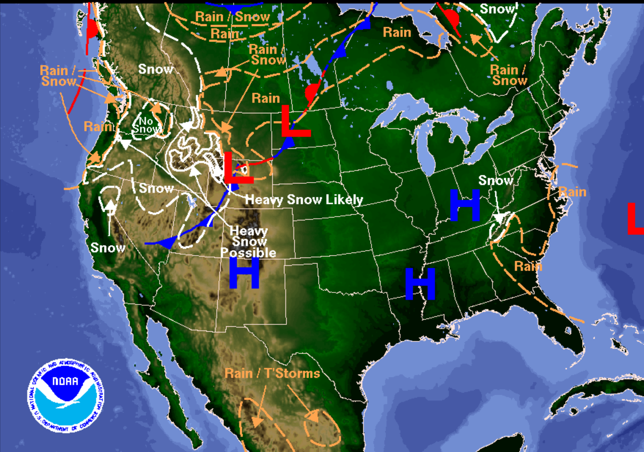
Weather Forecast for Tuesday, April 15, 2008 DOC/NOAA/NWS/NCEP/Hydrometeorological Prediction Center Prepared by Kong based on HPC, SPC, and TPC forecasts.
