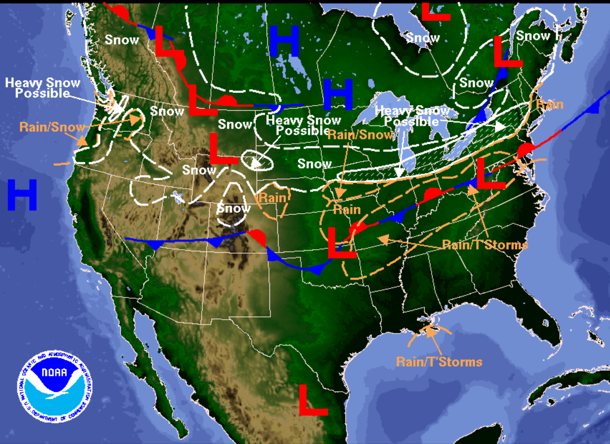
Weather Forecast for Thursday, March 27, 2008 DOC/NOAA/NWS/NCEP/Hydrometeorological Prediction Center Prepared by Kocin based on HPC, SPC, and TPC forecasts.
