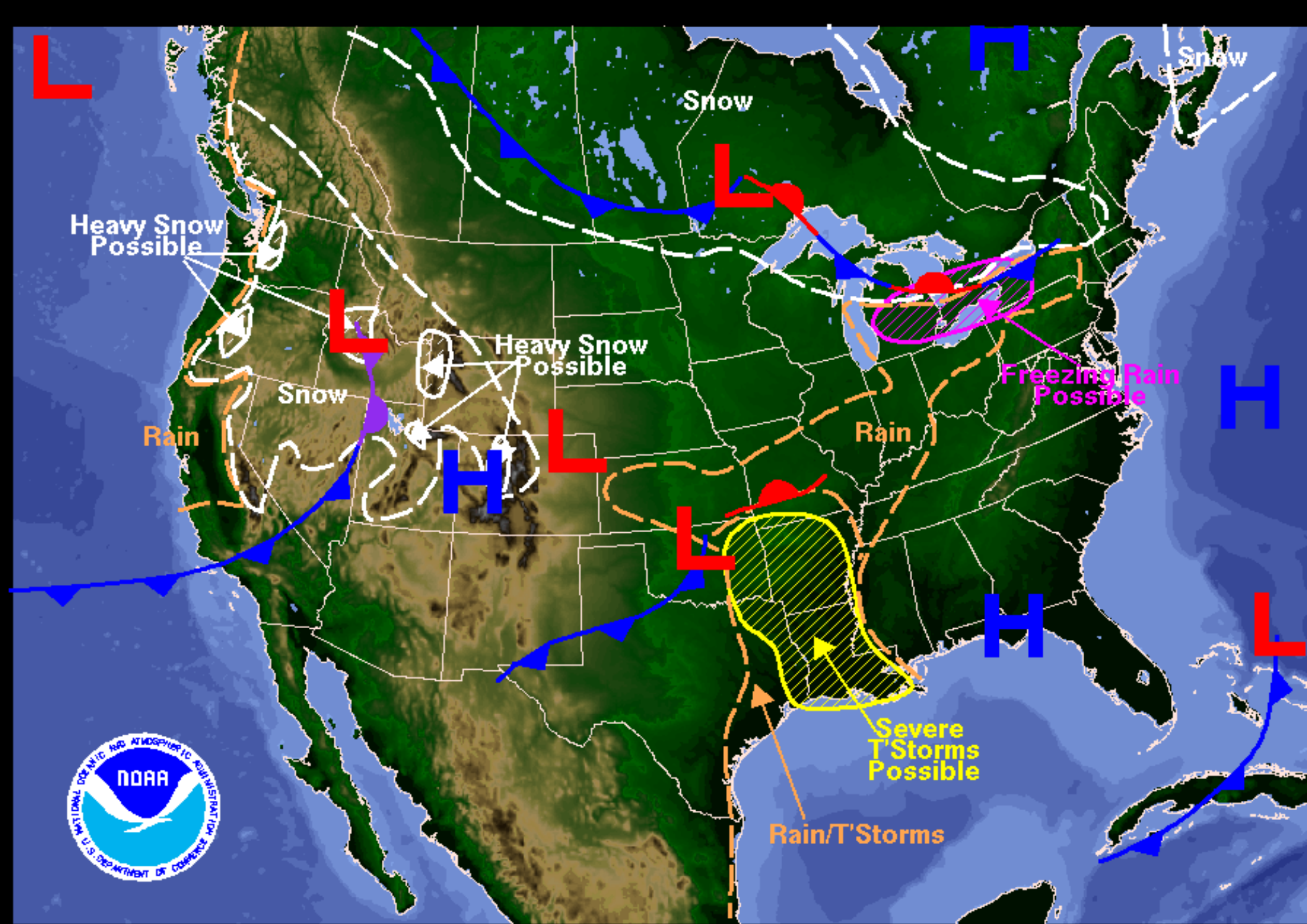
Weather Forecast for Thursday, March 13, 2008 DOC/NOAA/NWS/NCEP/Hydrometeorological Prediction Center Prepared by Collins based on HPC, SPC, and TPC forecasts.
