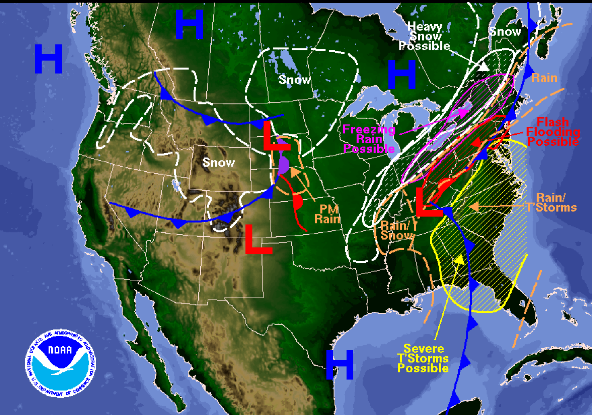
Weather Forecast for Tuesday, March 04, 2008 DOC/NOAA/NWS/NCEP/Hydrometeorological Prediction Center Prepared by Fracasso based on HPC, SPC, and TPC forecasts.
