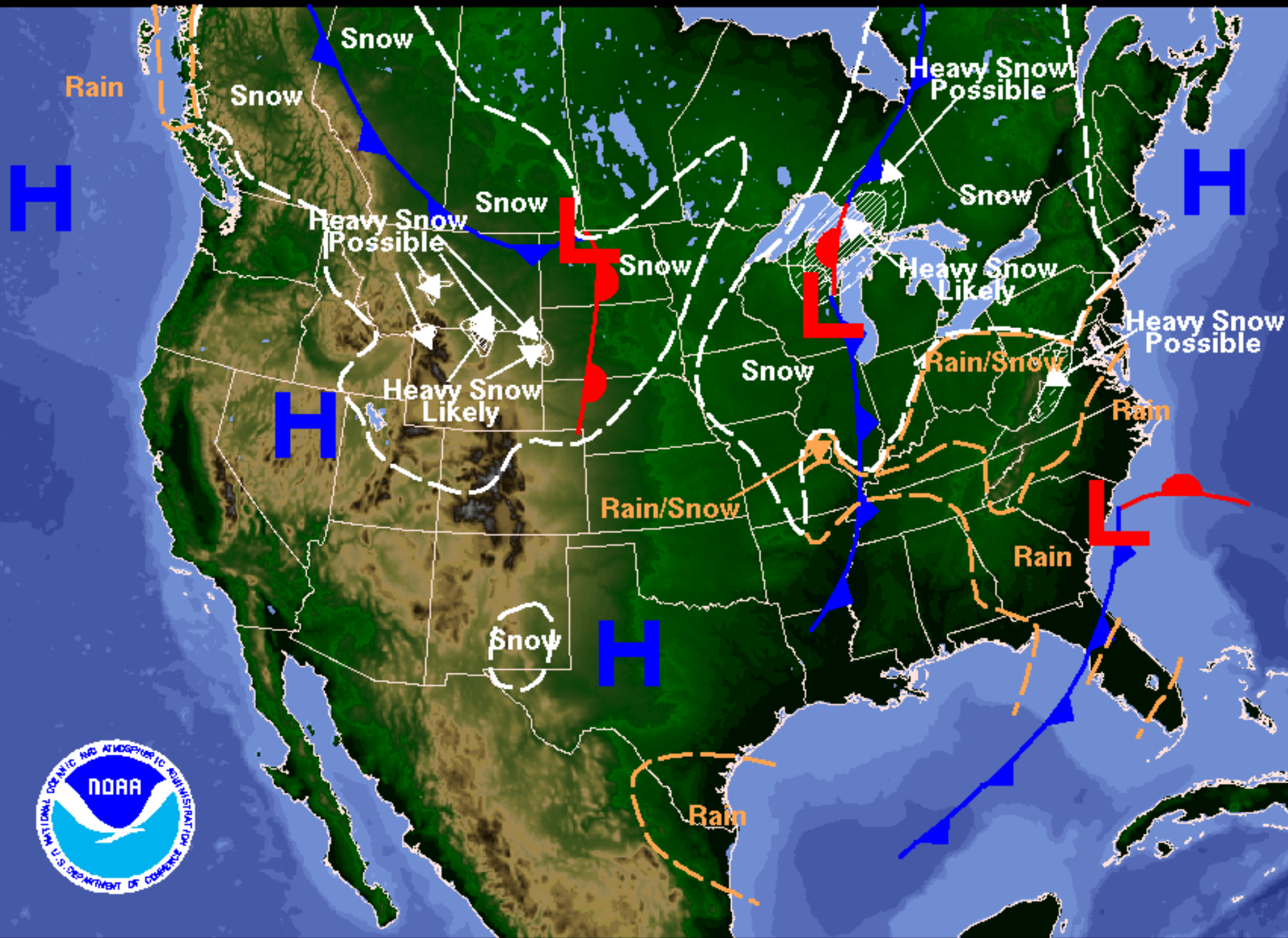
Weather Forecast for Thursday, January 17, 2008 DOC/NOAA/NWS/NCEP/Hydrometeorological Prediction Center Prepared by Kocin/Collins based on HPC, SPC, and TPC forecasts.
