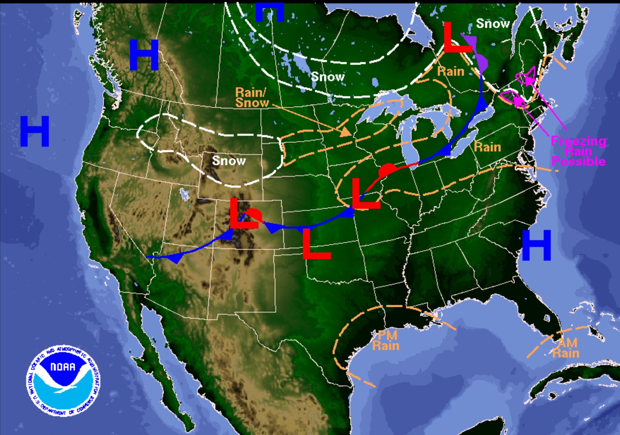
Weather Forecast for Tuesday, November 20, 2007 DOC/NOAA/NWS/NCEP/Hydrometeorological Prediction Center Prepared by Fracasso based on HPC, SPC, and TPC forecasts.
