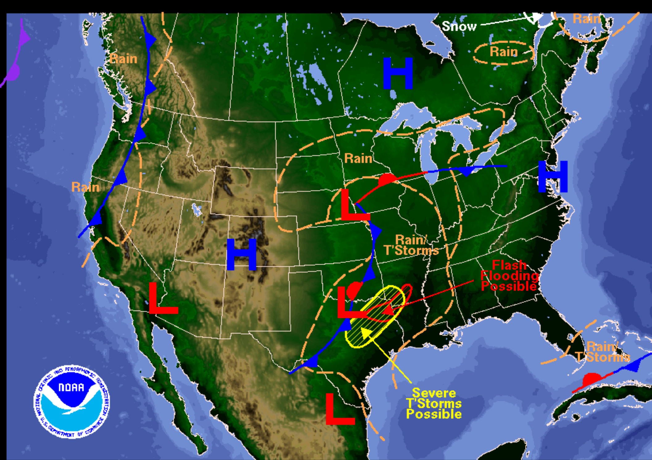
Weather Forecast for Monday, October 15, 2007 DOC/NOAA/NWS/NCEP/Hydrometeorological Prediction Center Prepared by Fracasso based on HPC, SPC, and TPC forecasts.
