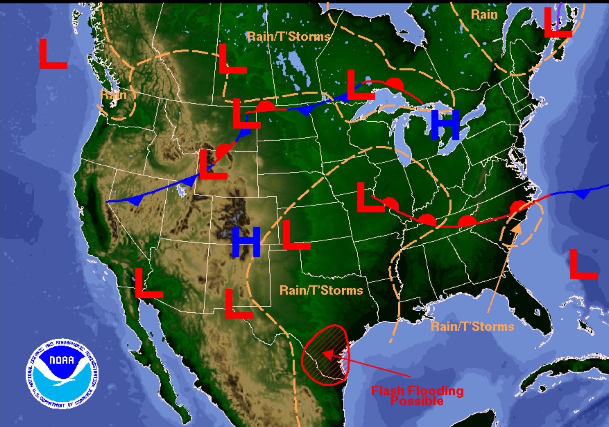
Weather Forecast for Saturday, June 23, 2007 DOC/NOAA/NWS/NCEP/Hydrometeorological Prediction Center Prepared by Otto based on HPC, SPC, and TPC forecasts.
