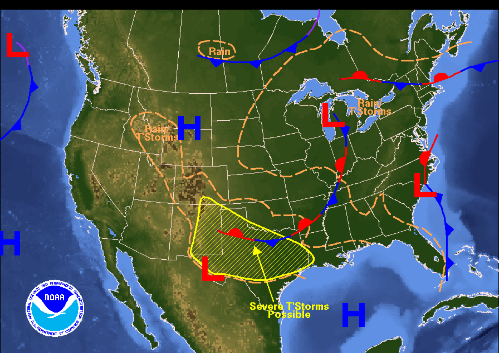
Weather Forecast for Sunday, June 03, 2007 DOC/NOAA/NWS/NCEP/Hydrometeorological Prediction Center Prepared by Rubin-Oster based on HPC, SPC, and TPC forecasts.
