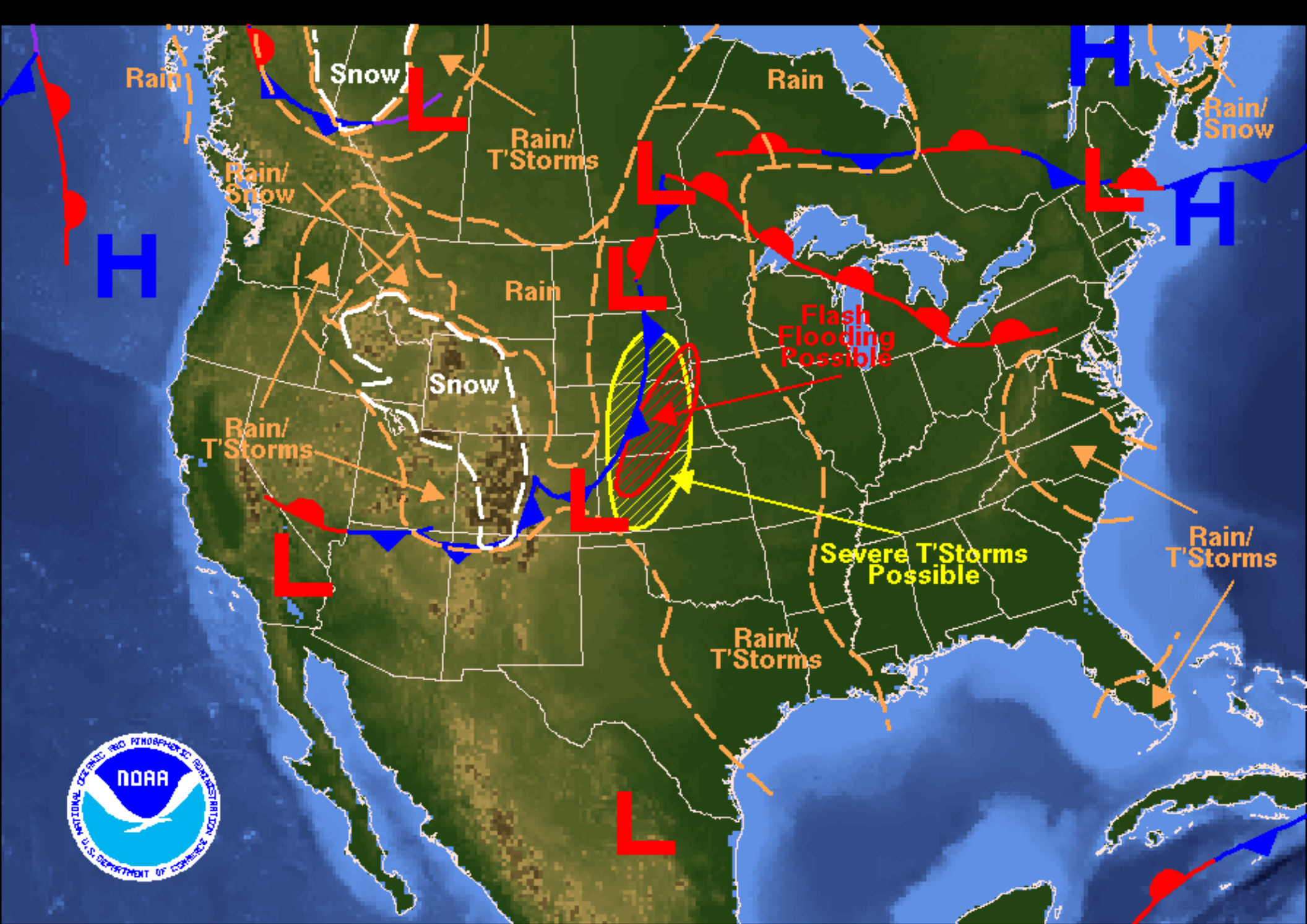
Weather Forecast for Tuesday, May 22, 2007 DOC/NOAA/NWS/NCEP/Hydrometeorological Prediction Center Prepared by Otto based on HPC, SPC, and TPC forecasts.
