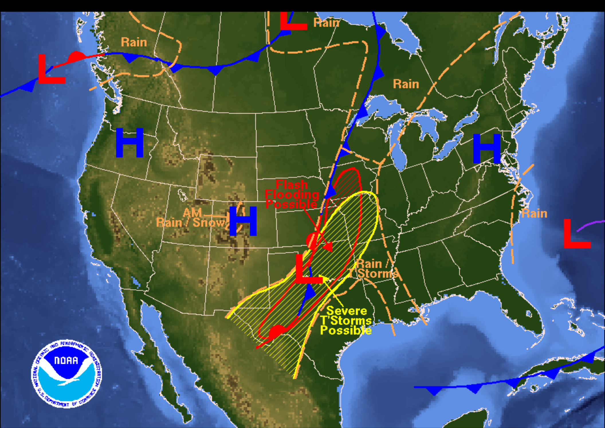
Weather Forecast for Monday, May 07, 2007 DOC/NOAA/NWS/NCEP/Hydrometeorological Prediction Center Prepared by Kong based on HPC, SPC, and TPC forecasts.
