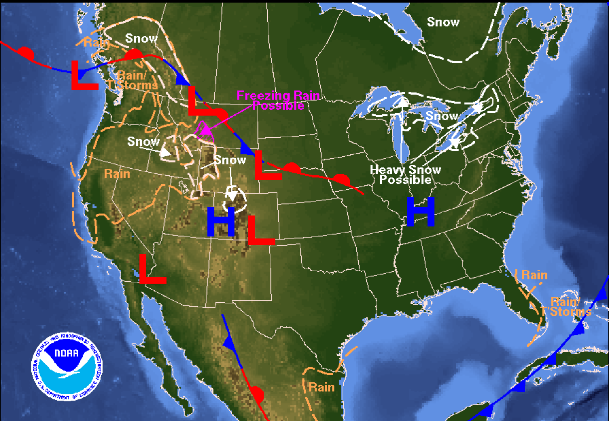
Weather Forecast for Friday, November 03, 2006 DOC/NOAA/NWS/NCEP/Hydrometeorological Prediction Center Prepared by Rubin-Oster based on HPC, SPC, and TPC forecasts.
