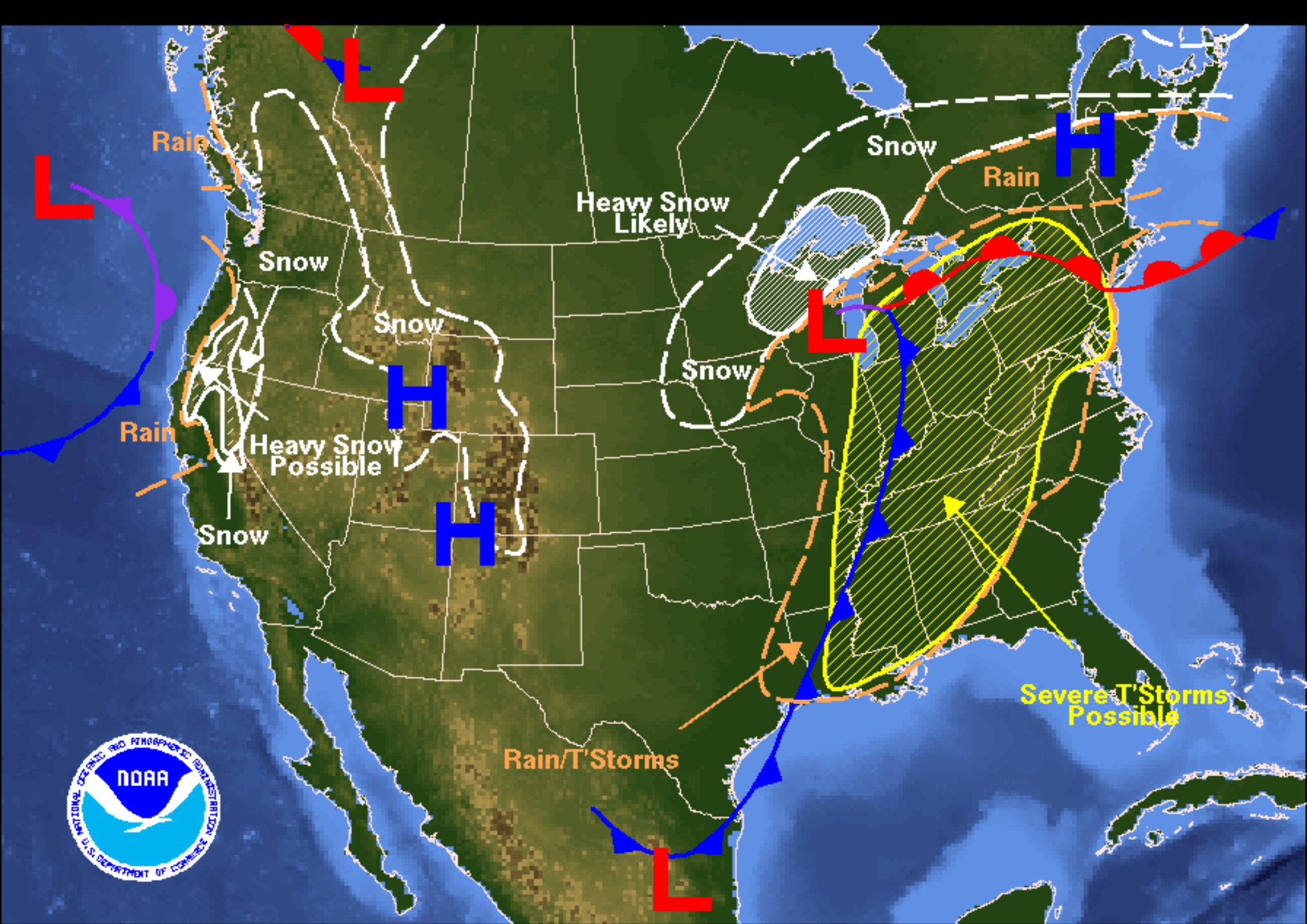
Weather Forecast for Monday, March 13, 2006 DOC/NOAA/NWS/NCEP/Hydrometeorological Prediction Center Prepared by Bell based on HPC, SPC, and TPC forecasts.
