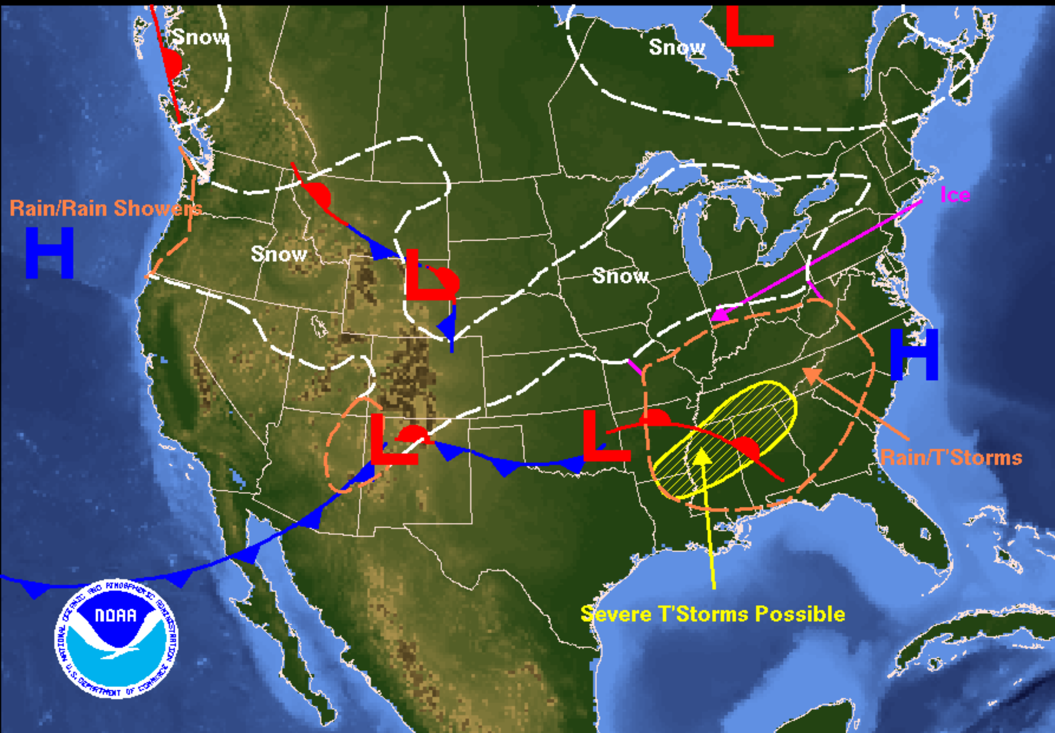
Weather Forecast for Saturday, December 03, 2005 DOC/NOAA/NWS/NCEP/Hydrometeorological Prediction Center Prepared by Kimberlain/Terry based on HPC, SPC, and TPC forecasts.
