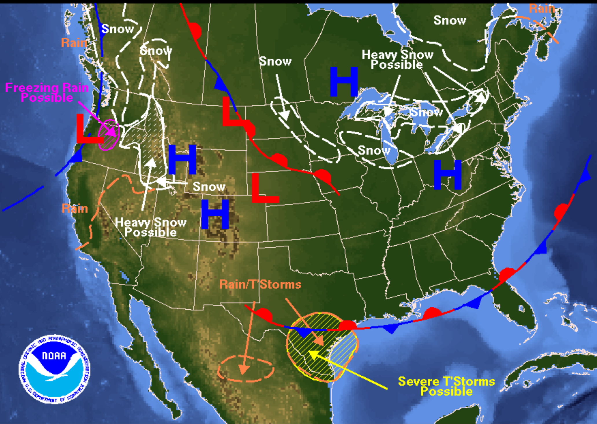
Weather Forecast for Friday, November 25, 2005 DOC/NOAA/NWS/NCEP/Hydrometeorological Prediction Center Prepared by Bell/Eckert based on HPC, SPC, and TPC forecasts.
