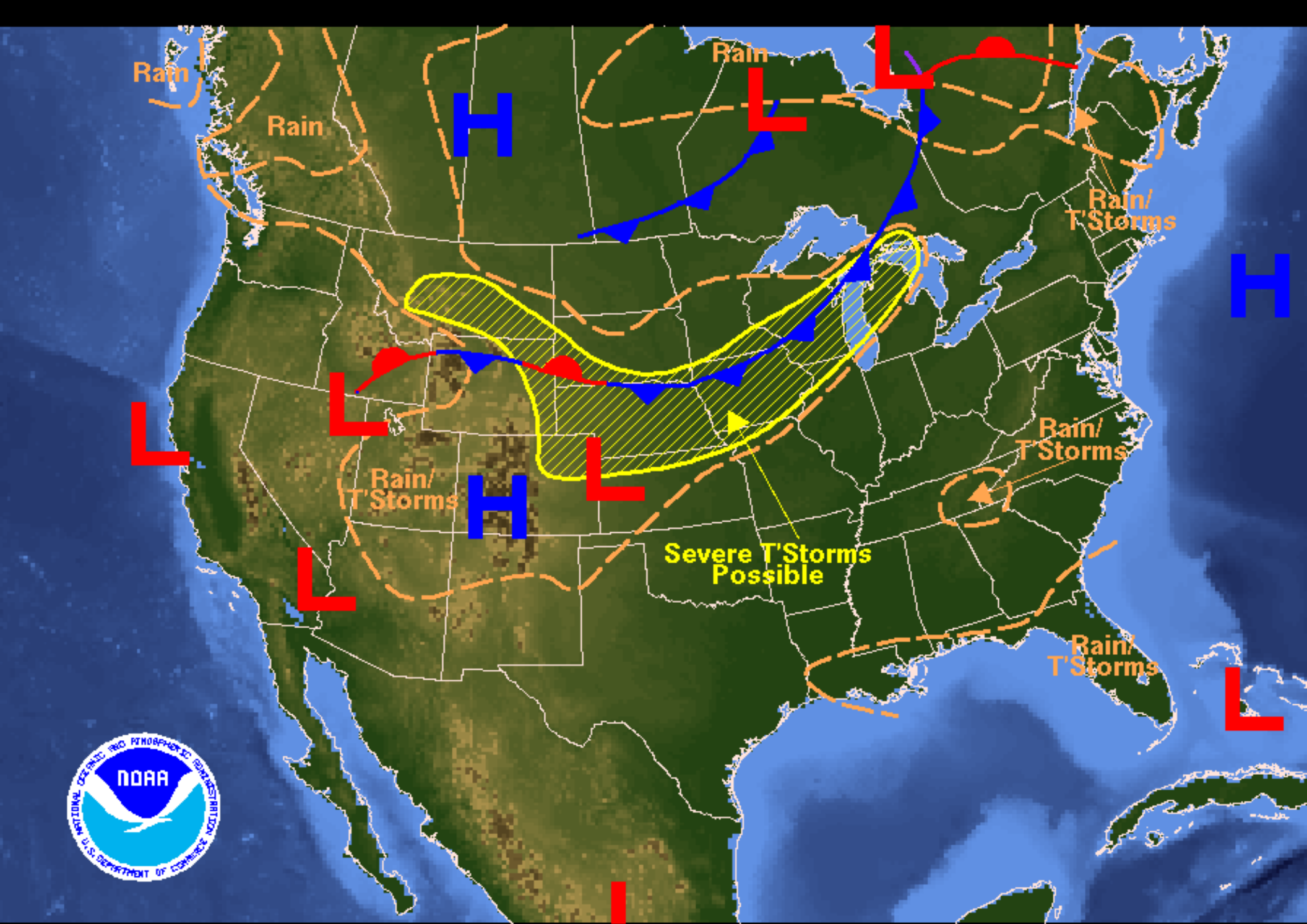
Weather Forecast for Friday, June 24, 2005 DOC/NOAA/NWS/NCEP/Hydrometeorological Prediction Center Prepared by Fries/Sullivan based on HPC, SPC, and TPC forecasts.
