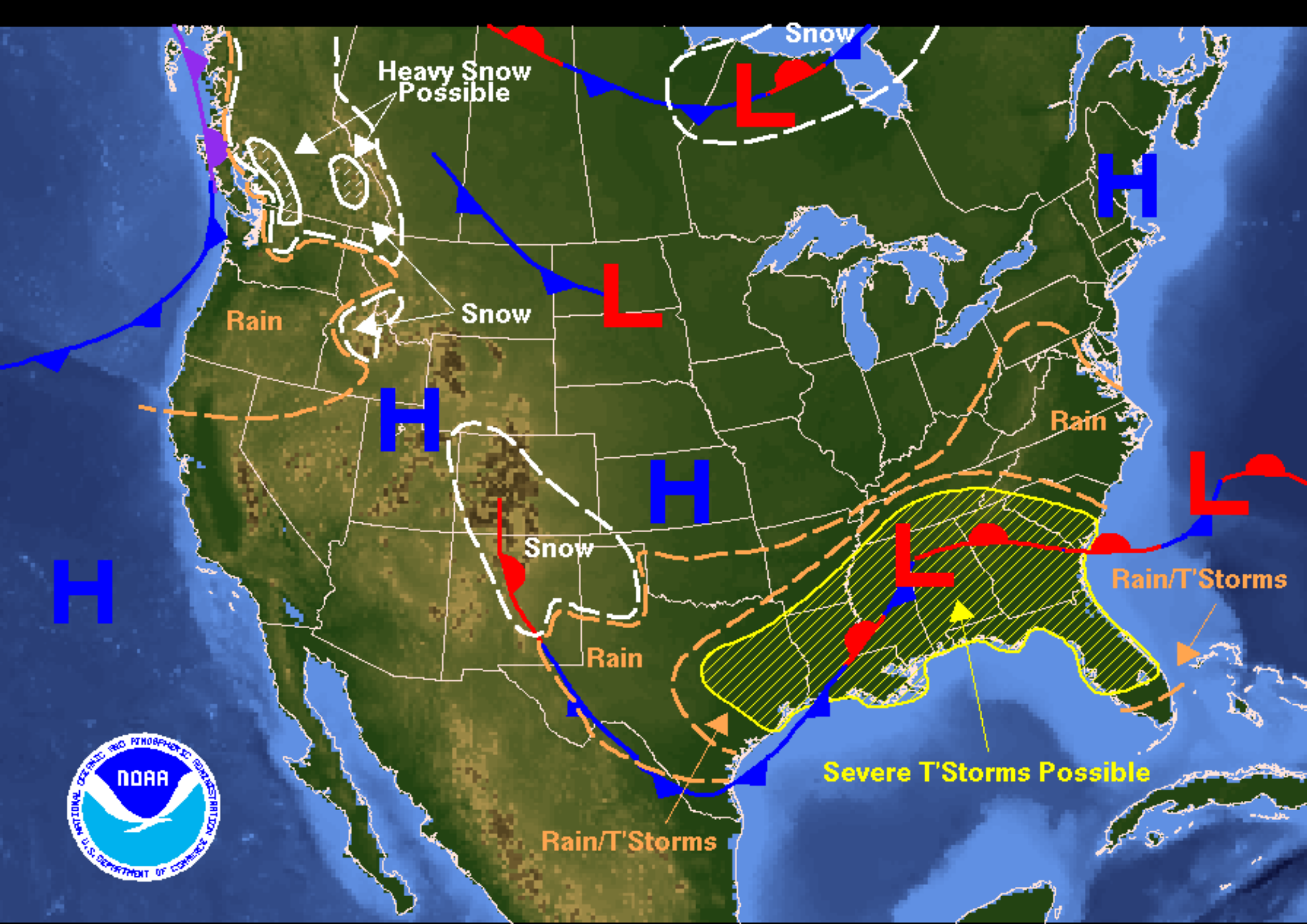
Weather Forecast for Saturday, March 26, 2005 DOC/NOAA/NWS/NCEP/Hydrometeorological Prediction Center Prepared by Szataneck/Eckert based on HPC, SPC, and TPC forecasts.
