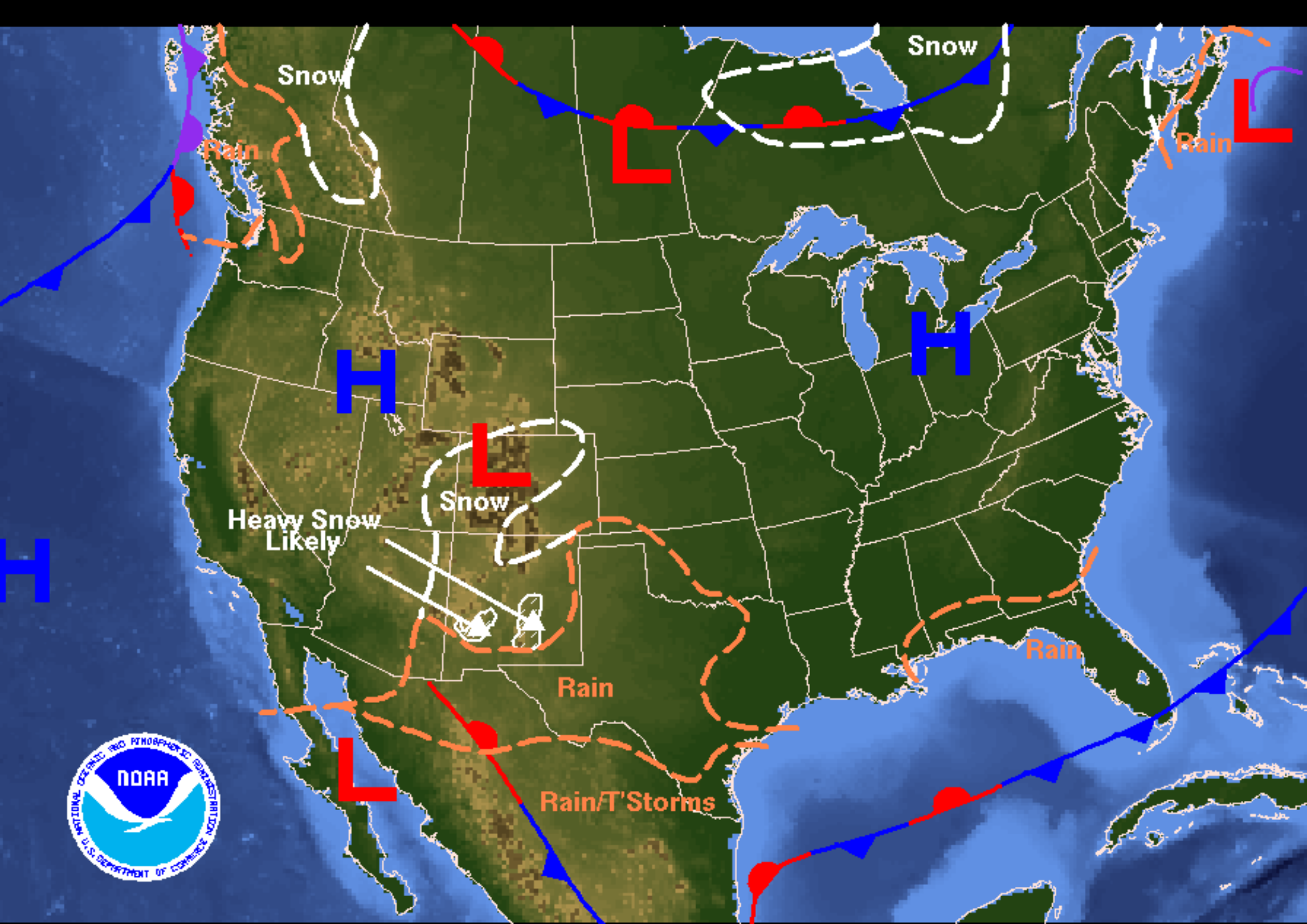
Weather Forecast for Sunday, November 14, 2004 DOC/NOAA/NWS/NCEP/Hydrometeorological Prediction Center Prepared by Bell/Terry based on HPC, SPC, and TPC forecasts.
