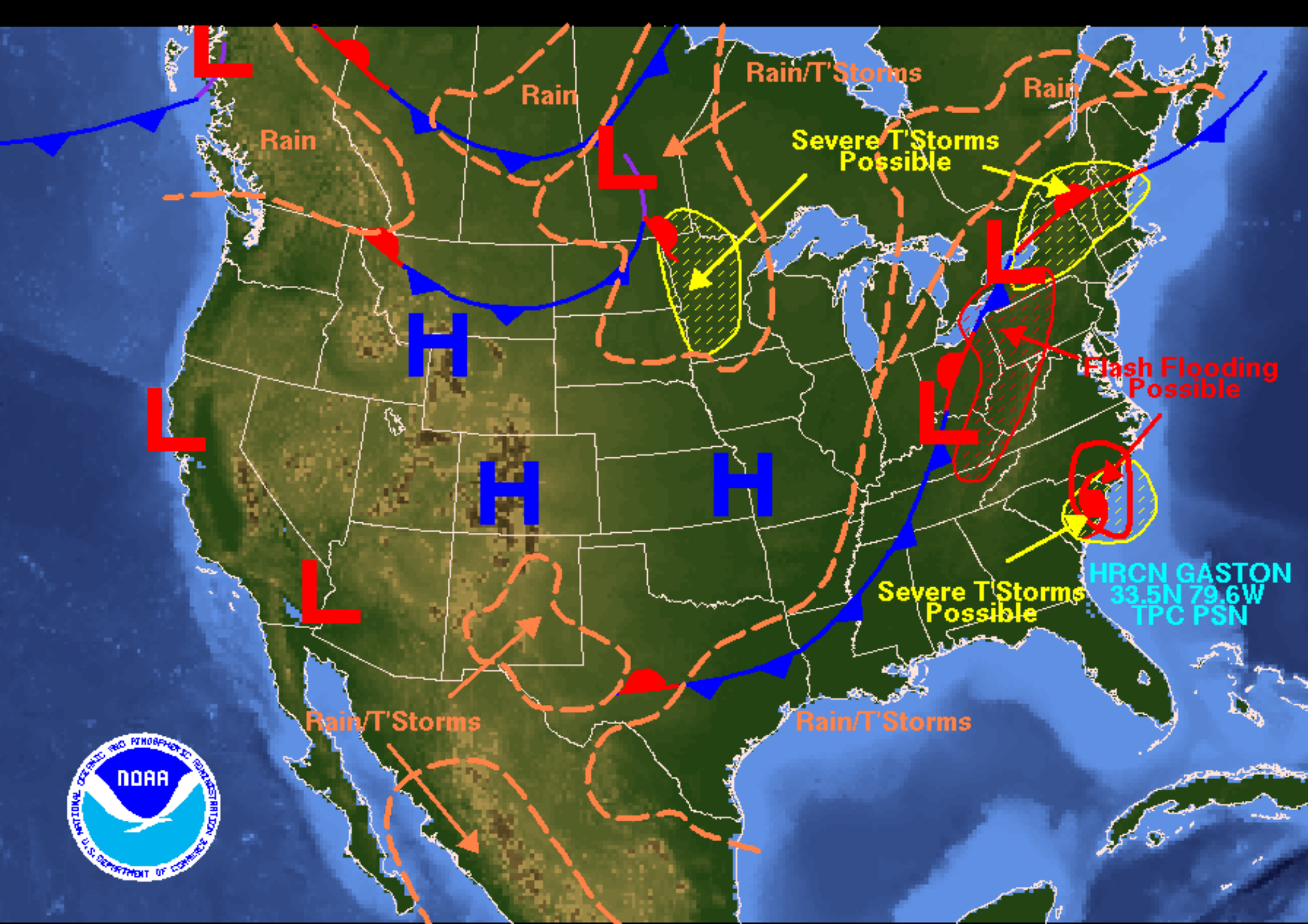
Weather Forecast for Sunday, August 29, 2004 DOC/NOAA/NWS/NCEP/Hydrometeorological Prediction Center Prepared by Bell/Eckert based on HPC, SPC, and TPC forecasts.
